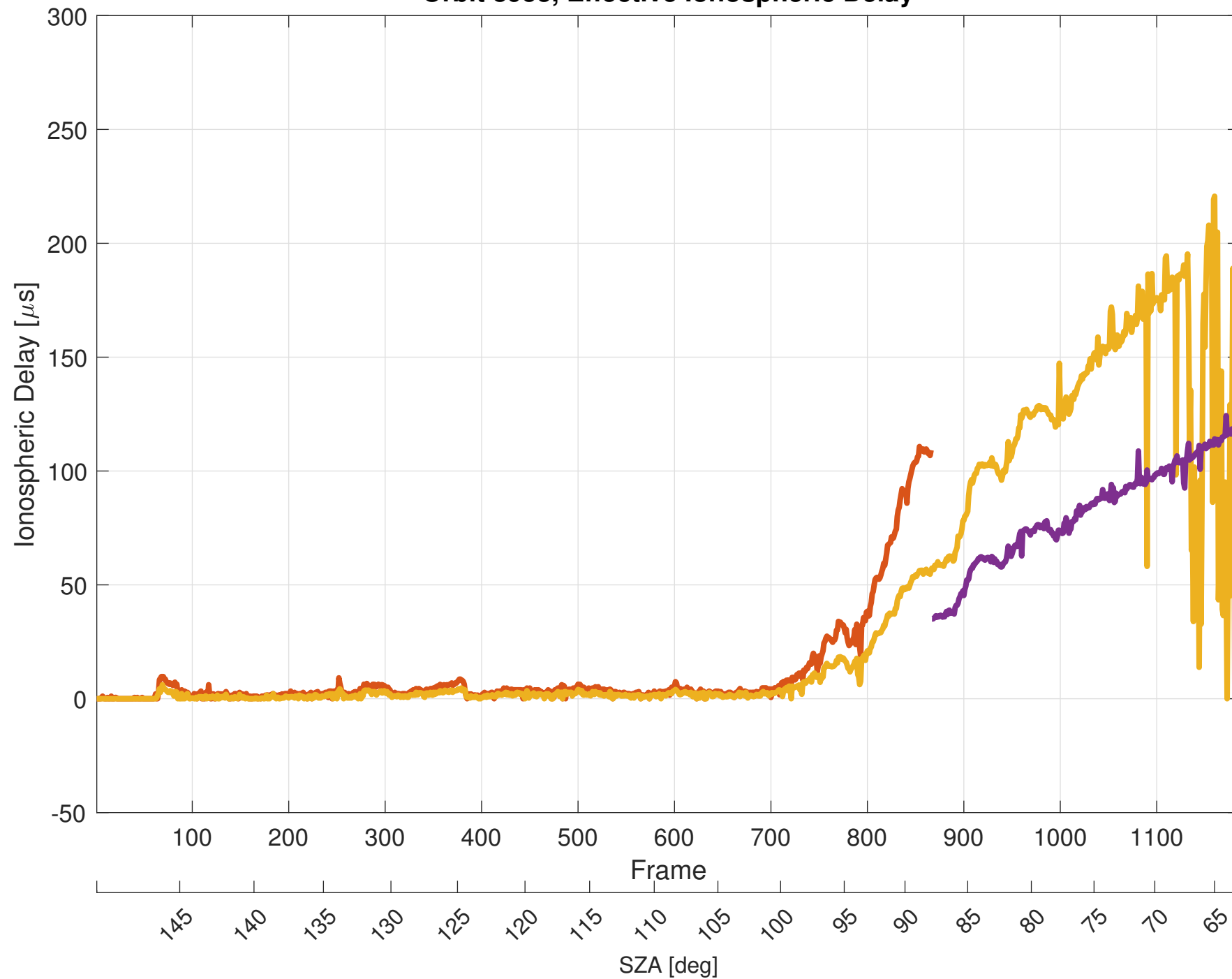
Orbit 8953, Effective Ionospheric Delay
