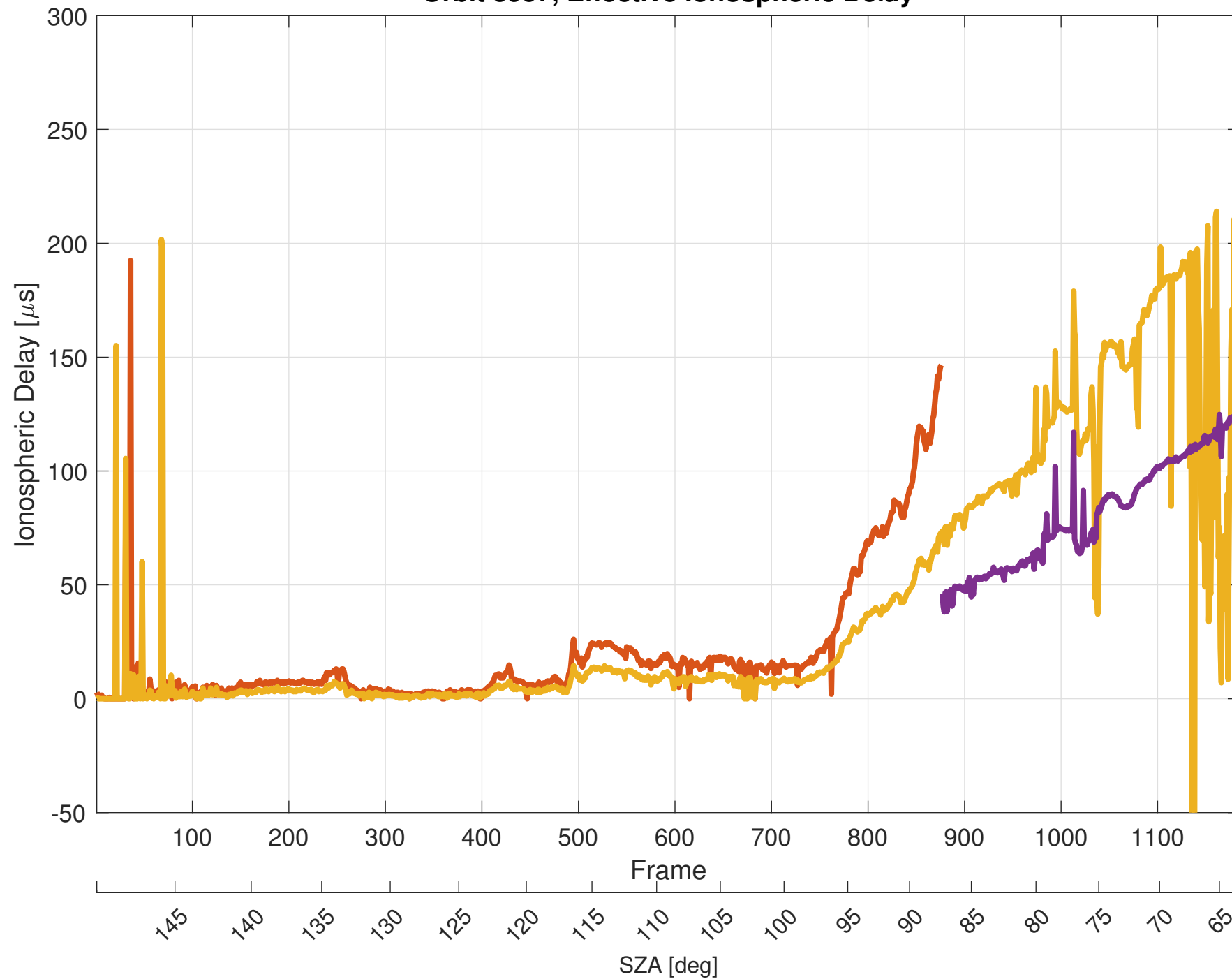
Orbit 8957, Effective Ionospheric Delay
