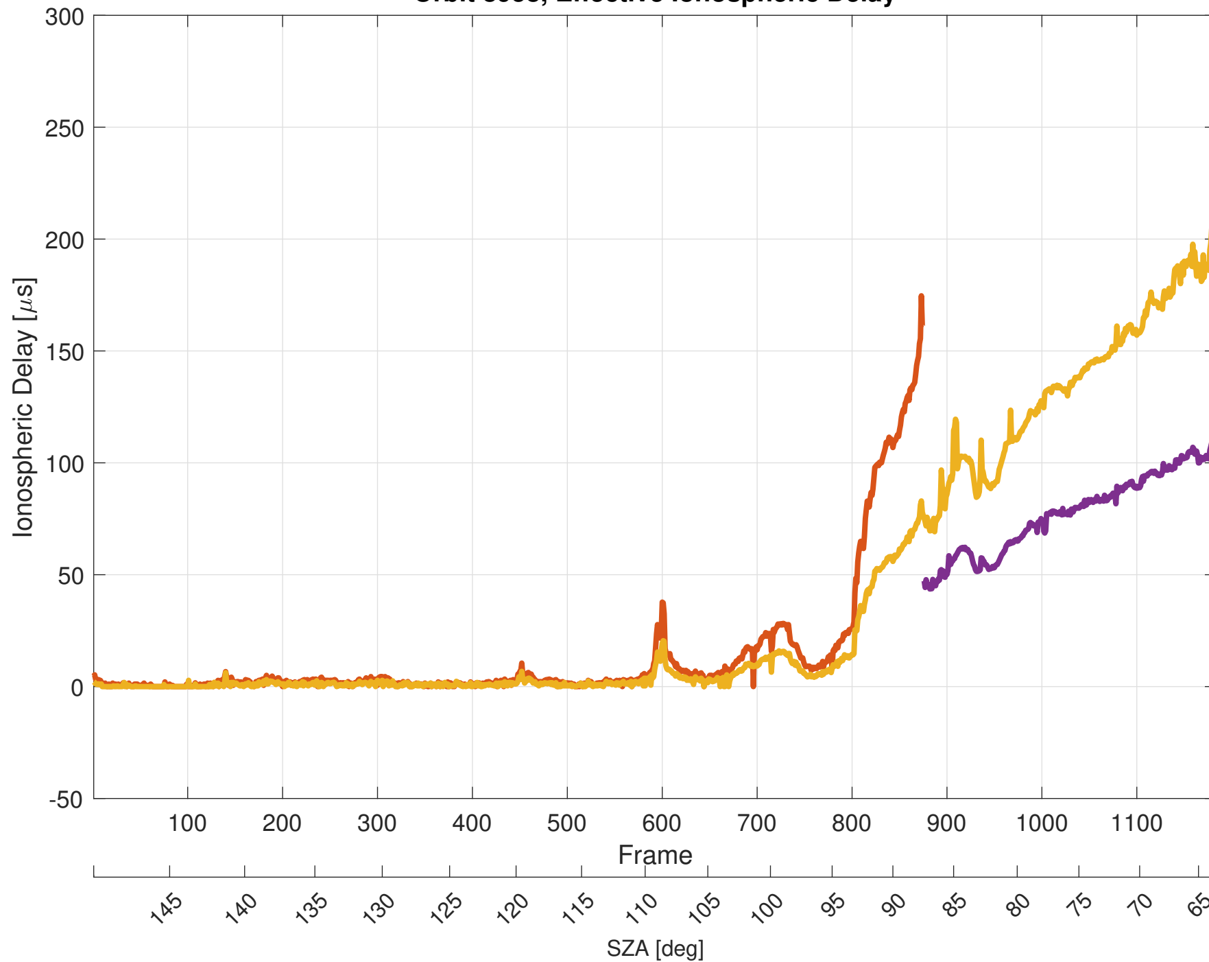
Orbit 8958, Effective Ionospheric Delay
