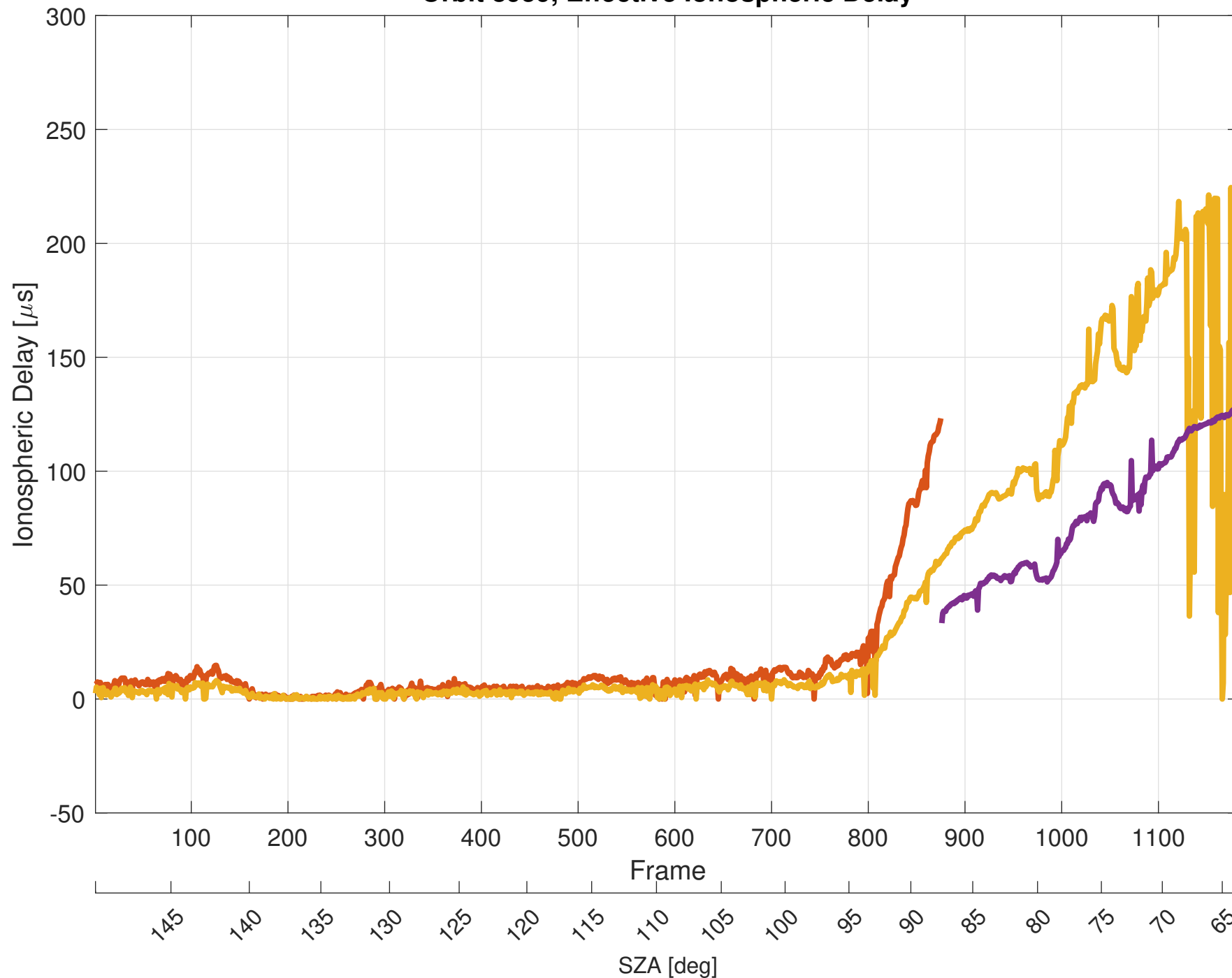
Orbit 8959, Effective Ionospheric Delay
