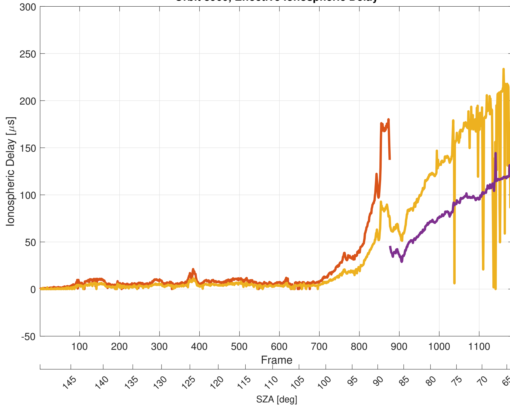
Orbit 8960, Effective Ionospheric Delay
