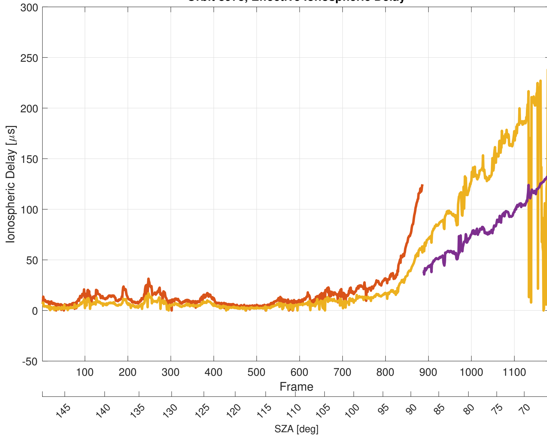
Orbit 8973, Effective Ionospheric Delay
