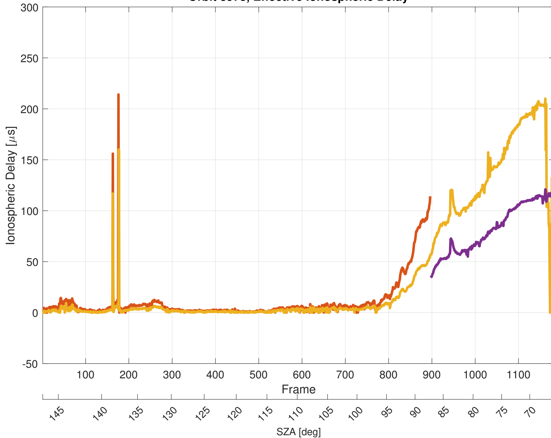
Orbit 8978, Effective Ionospheric Delay
