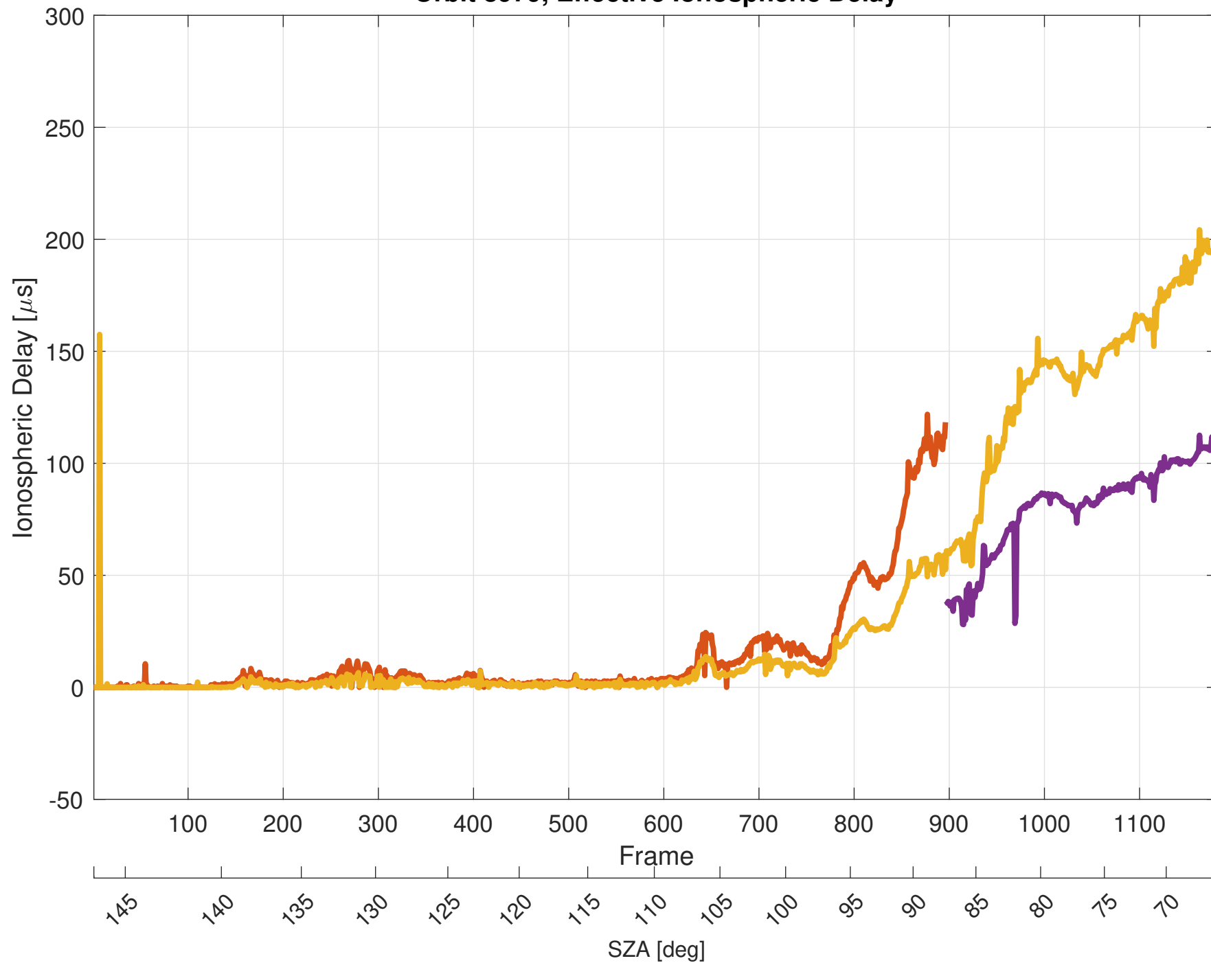
Orbit 8979, Effective Ionospheric Delay
