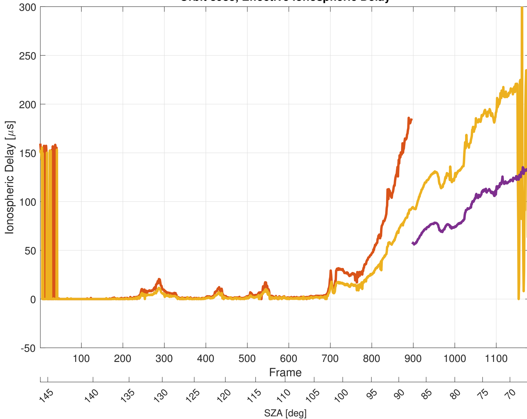
Orbit 8983, Effective Ionospheric Delay
