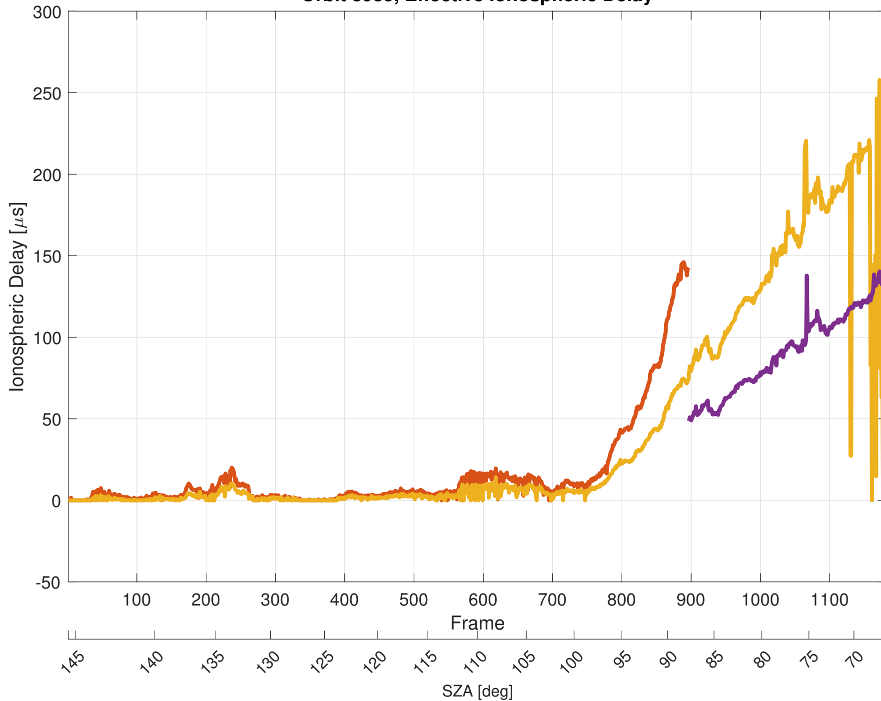
Orbit 8985, Effective Ionospheric Delay
