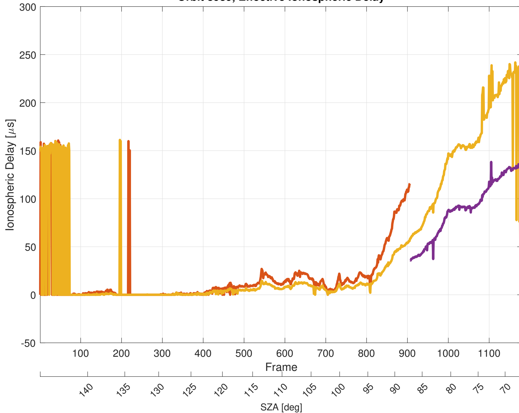
Orbit 8989, Effective Ionospheric Delay
