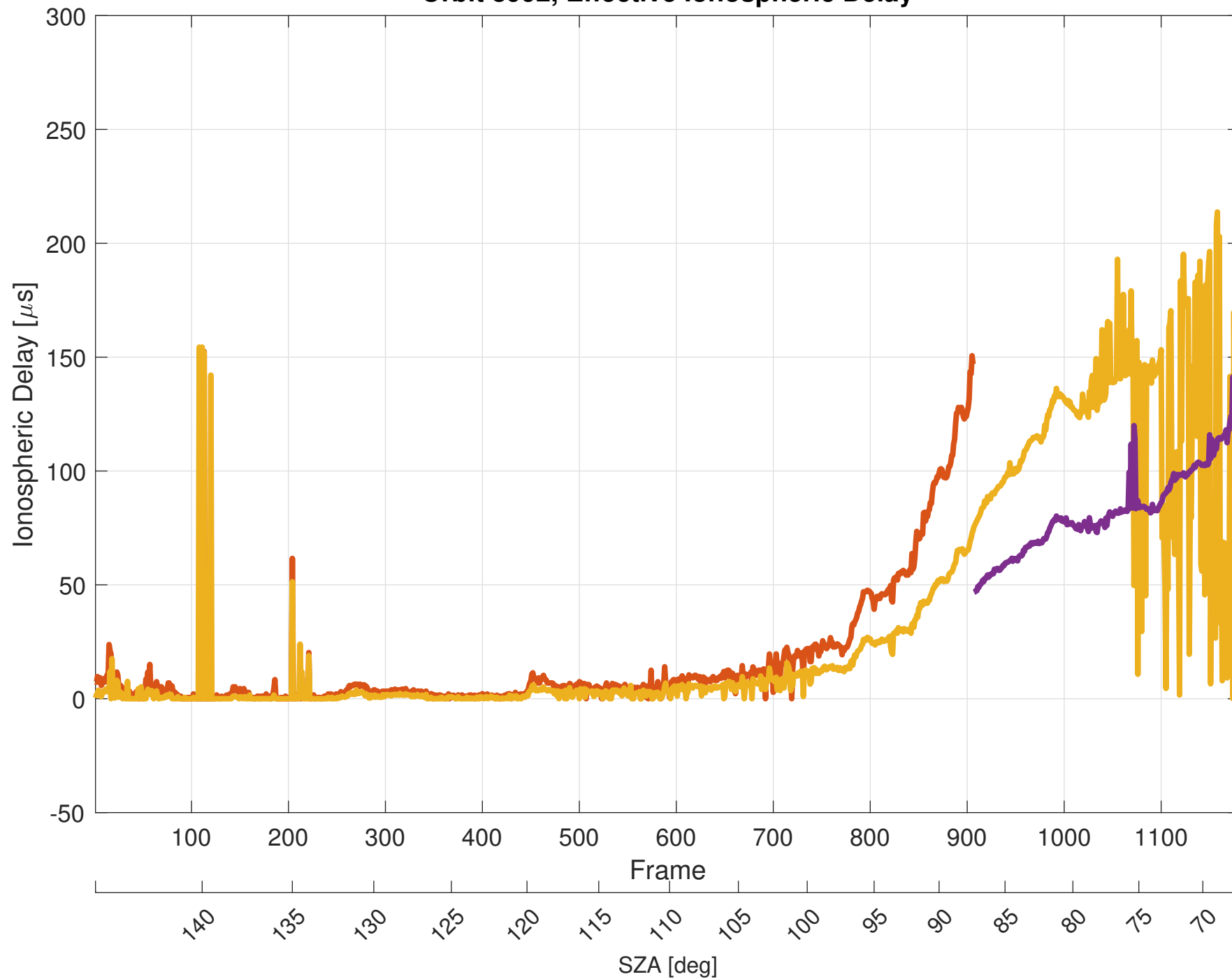
Orbit 8992, Effective Ionospheric Delay
