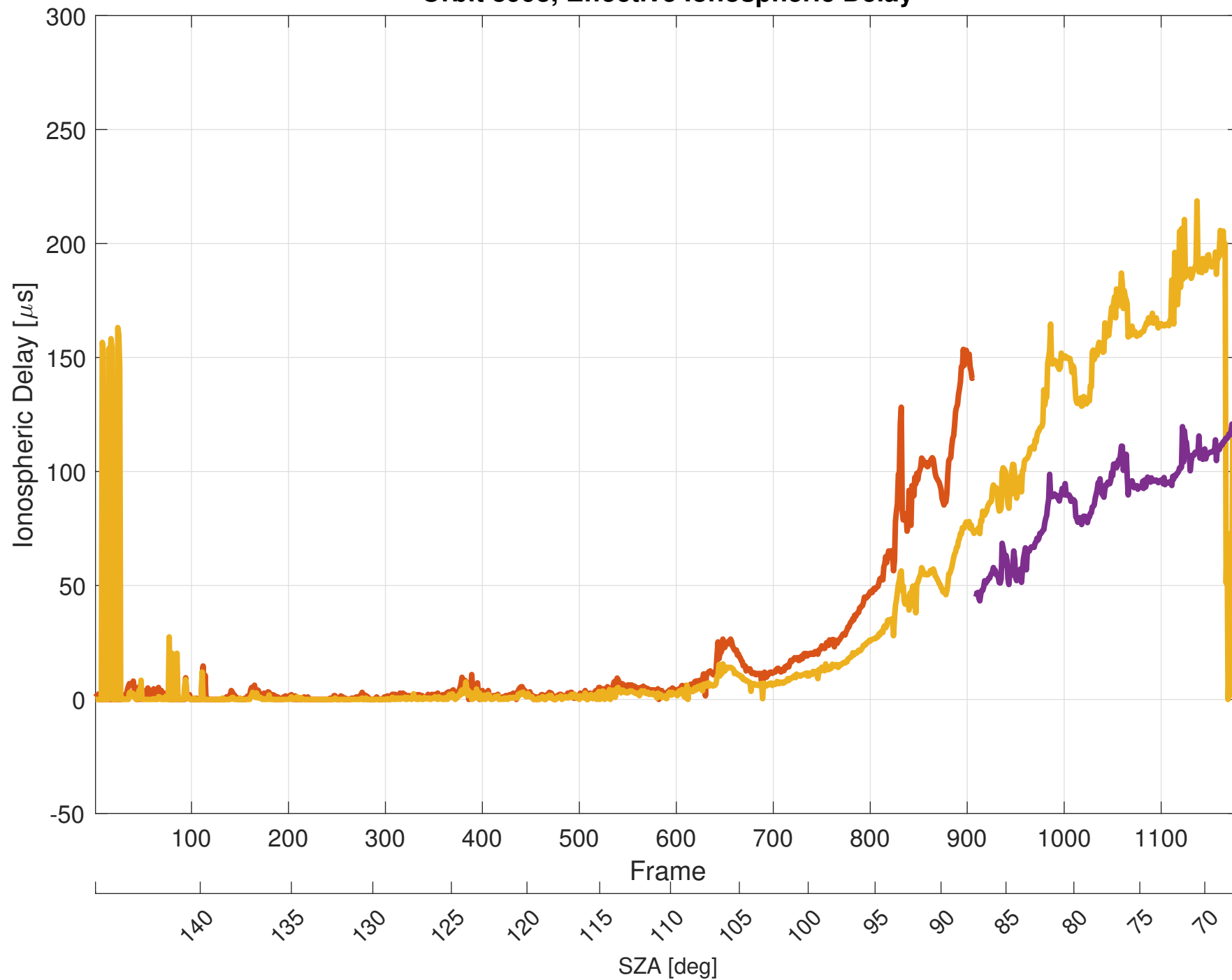
Orbit 8993, Effective Ionospheric Delay
