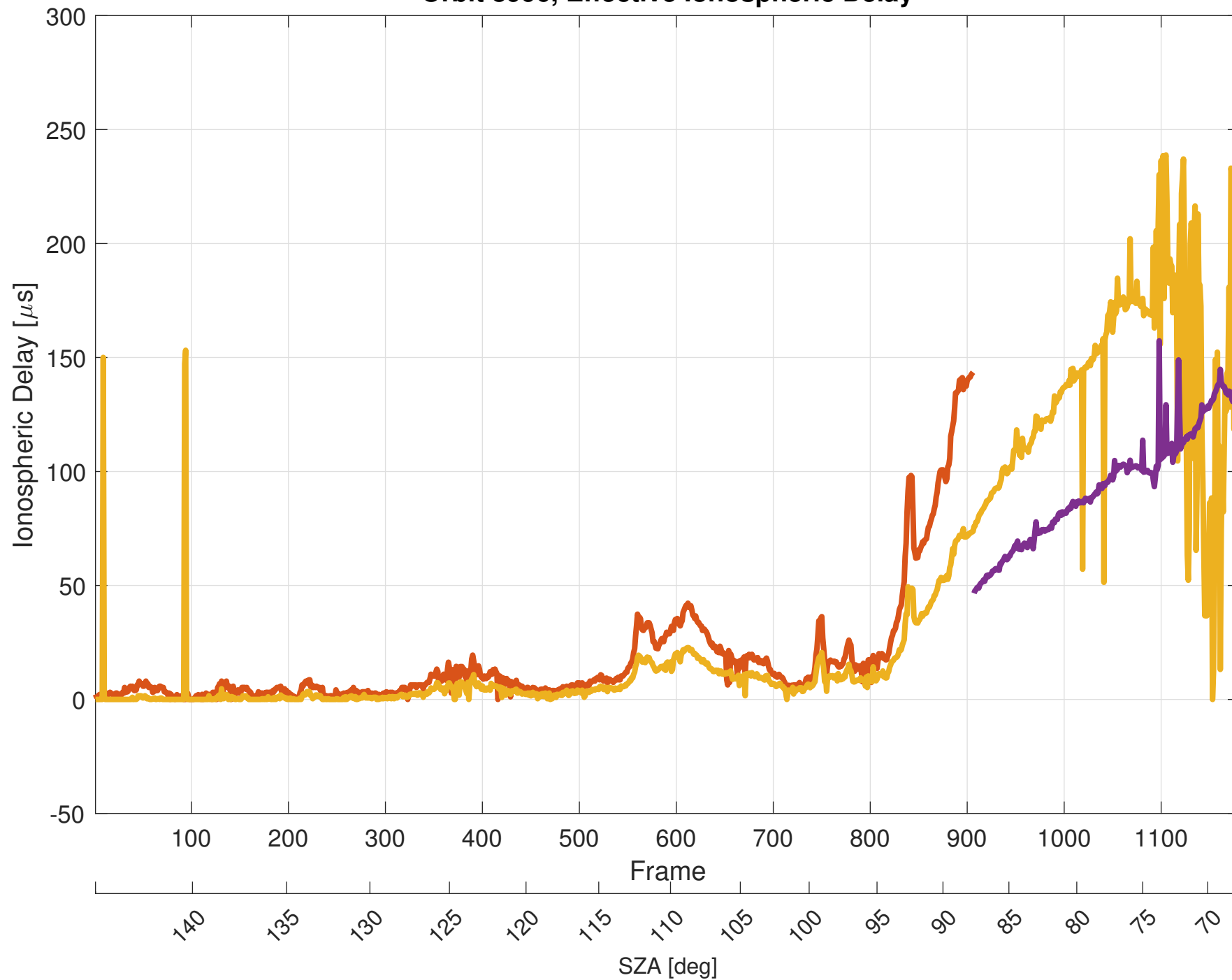
Orbit 8996, Effective Ionospheric Delay
