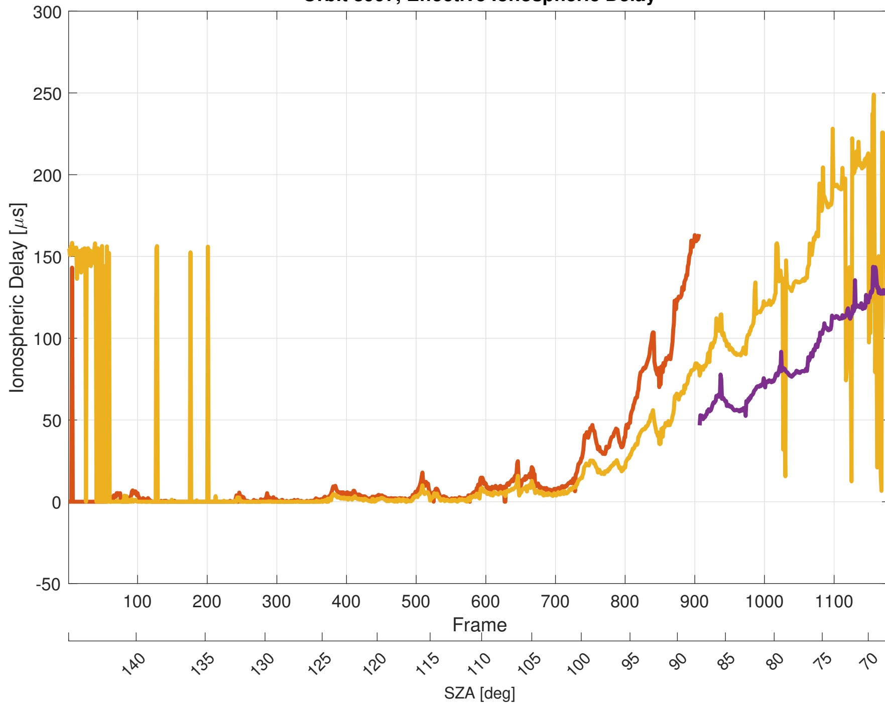
Orbit 8997, Effective Ionospheric Delay
