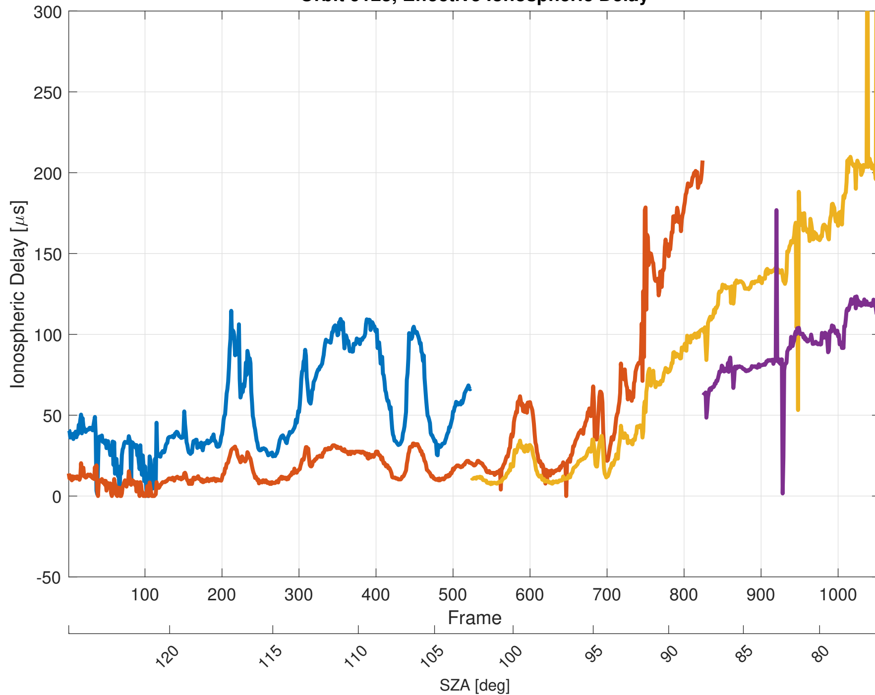
Orbit 9123, Effective Ionospheric Delay
