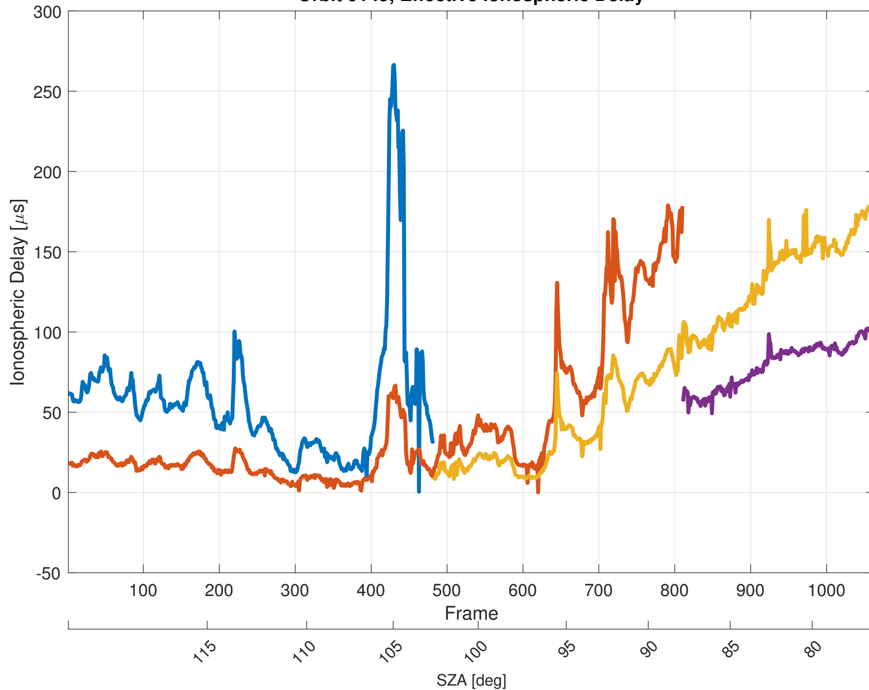
Orbit 9145, Effective Ionospheric Delay
