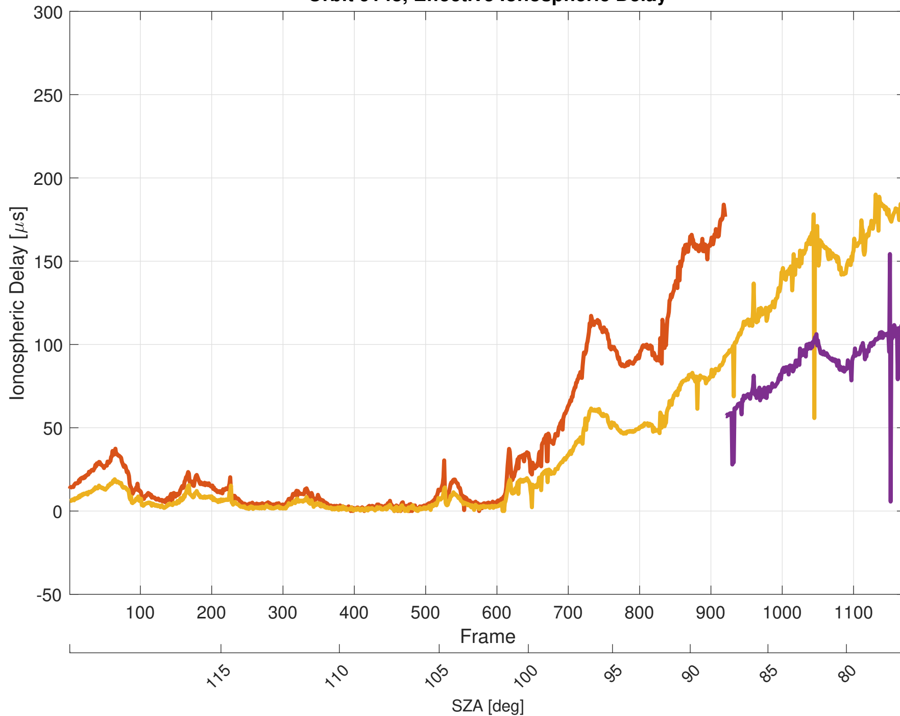
Orbit 9148, Effective Ionospheric Delay
