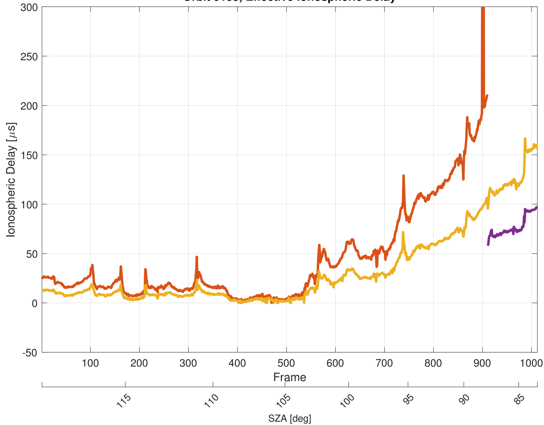
Orbit 9155, Effective Ionospheric Delay
