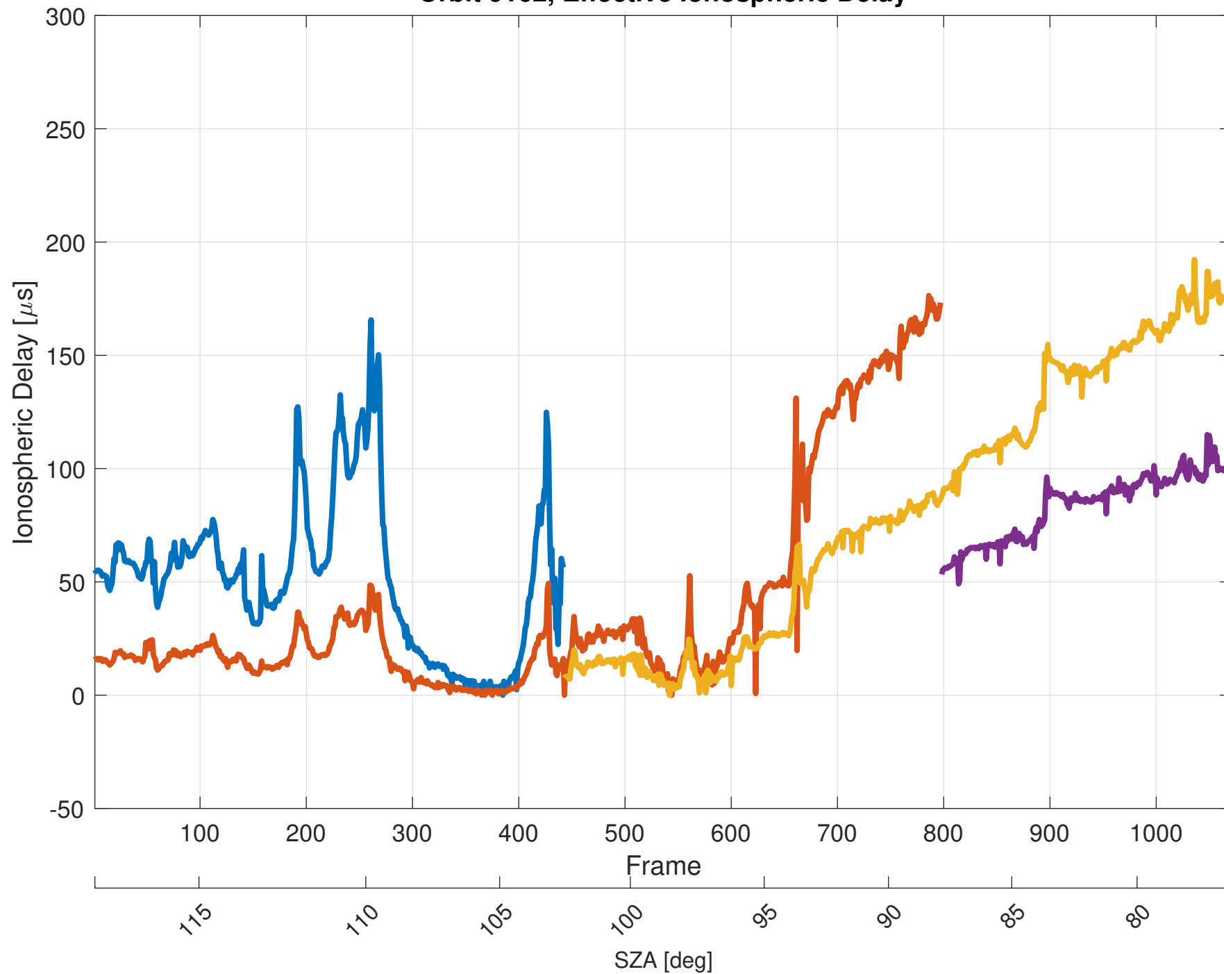
Orbit 9162, Effective Ionospheric Delay
