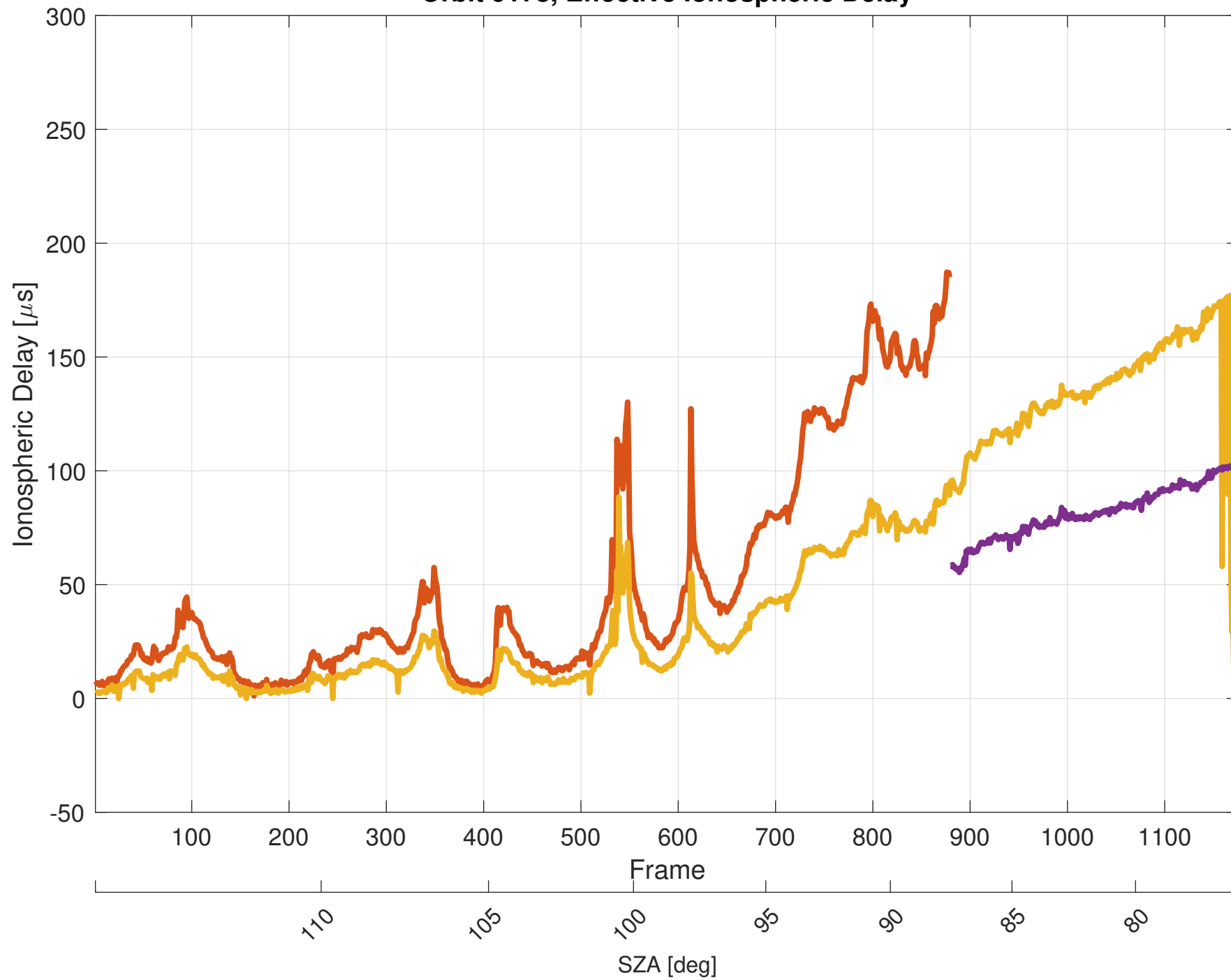
Orbit 9178, Effective Ionospheric Delay
