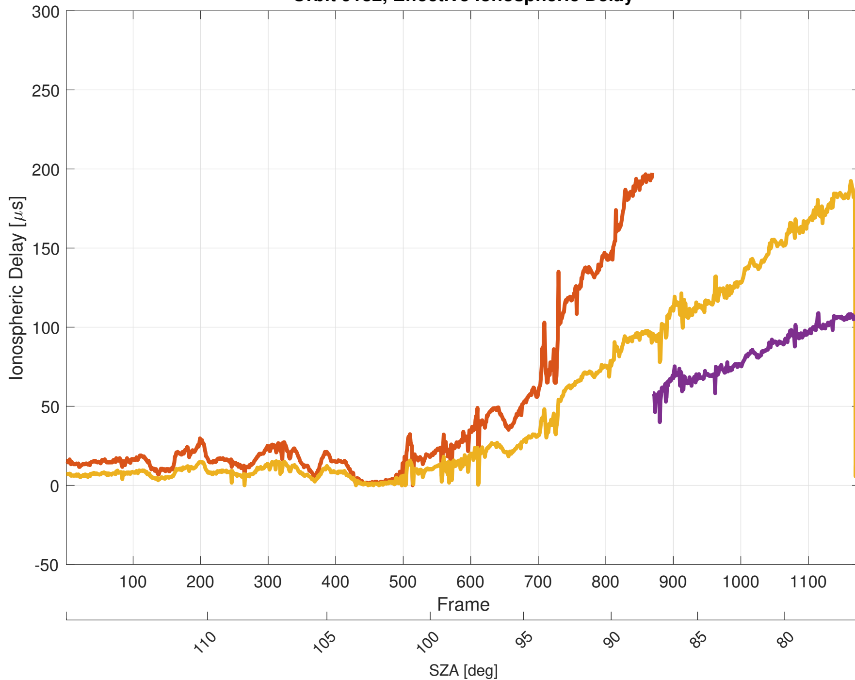
Orbit 9182, Effective Ionospheric Delay
