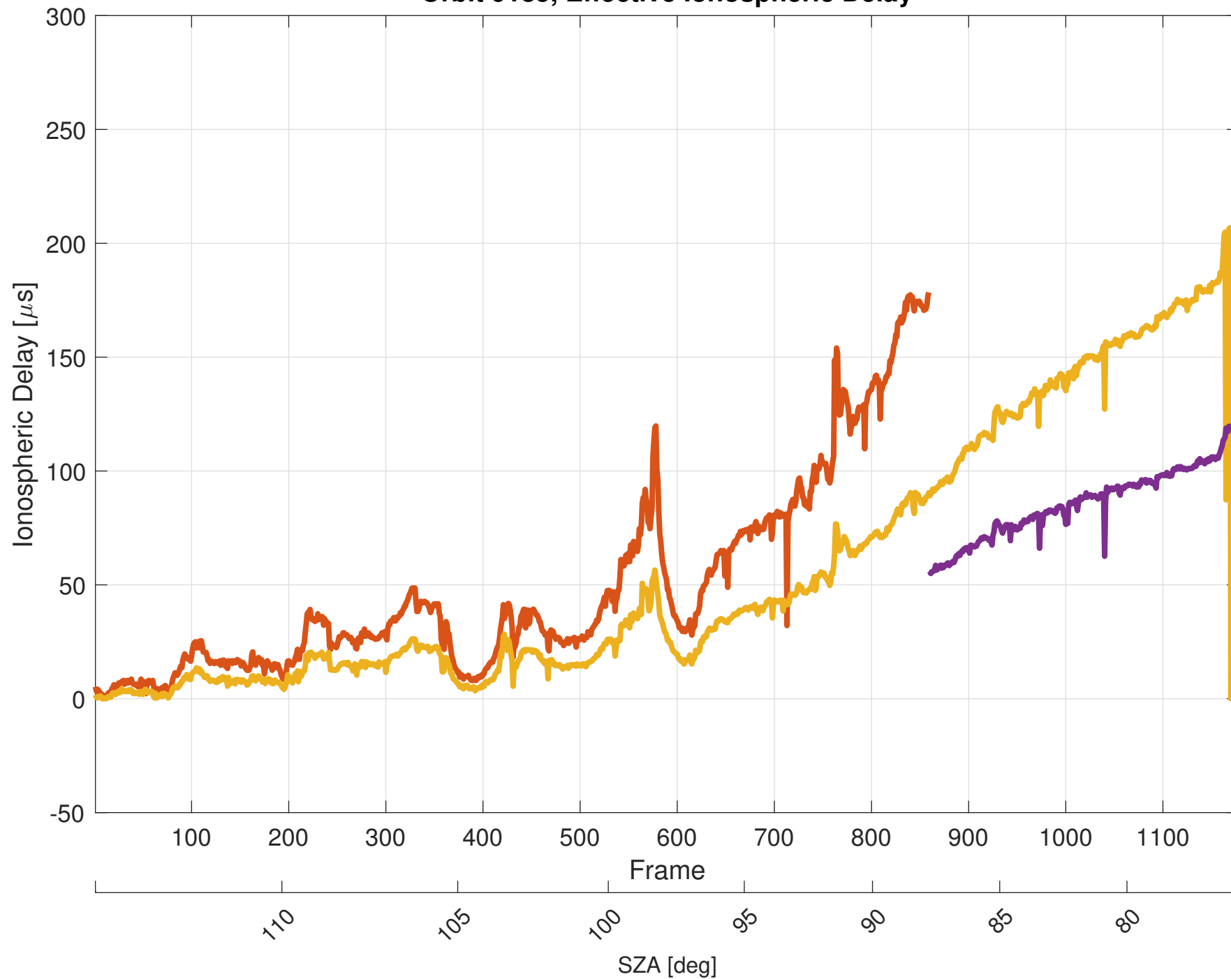
Orbit 9185, Effective Ionospheric Delay
