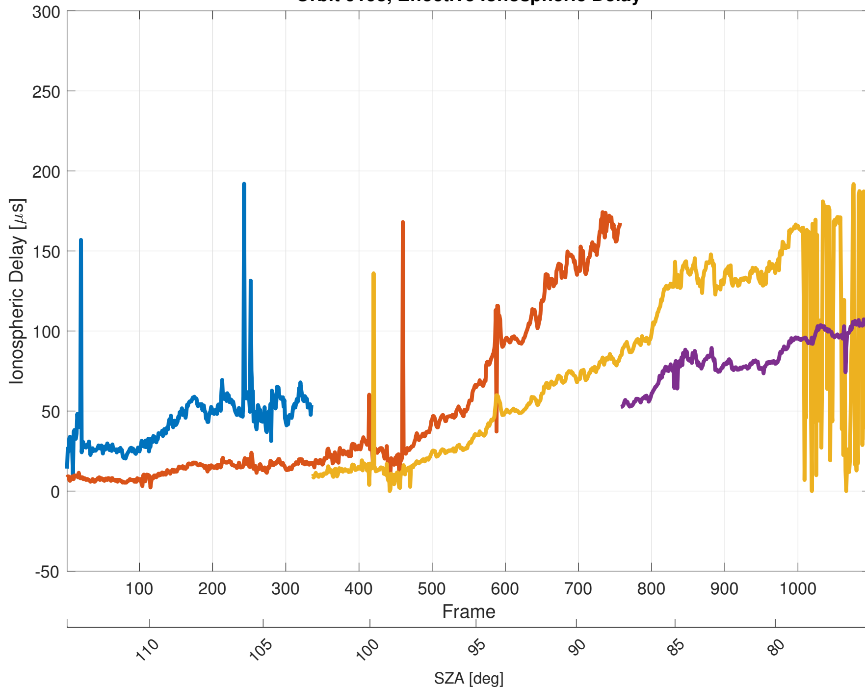
Orbit 9193, Effective Ionospheric Delay
