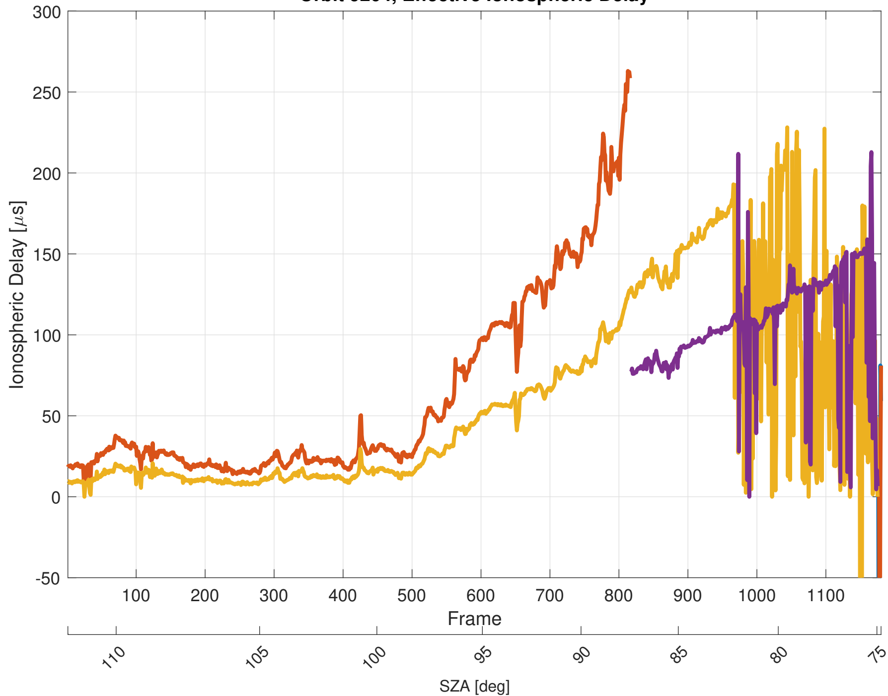
Orbit 9204, Effective Ionospheric Delay
