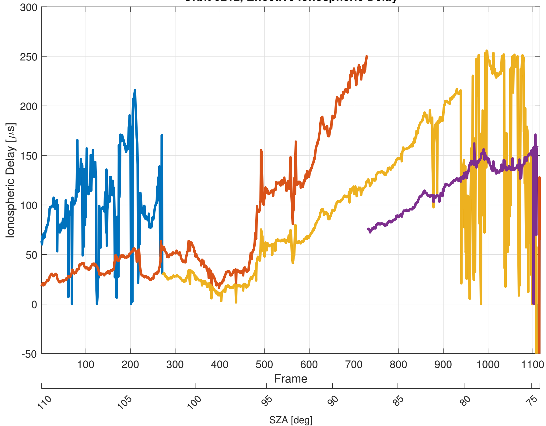
Orbit 9212, Effective Ionospheric Delay
