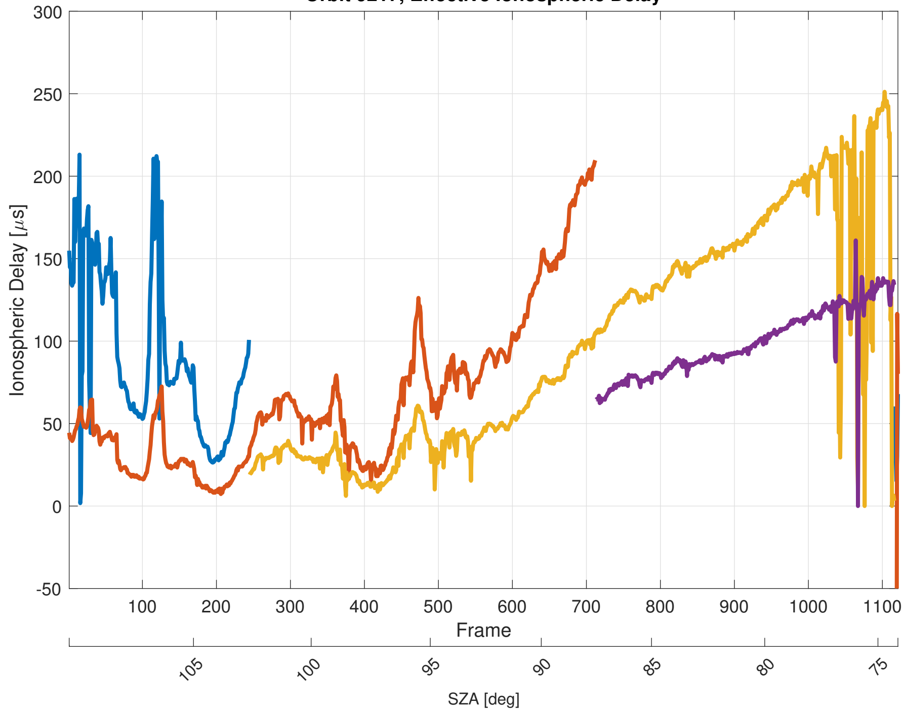
Orbit 9217, Effective Ionospheric Delay
