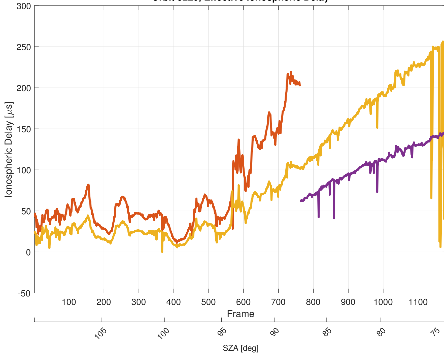
Orbit 9220, Effective Ionospheric Delay
