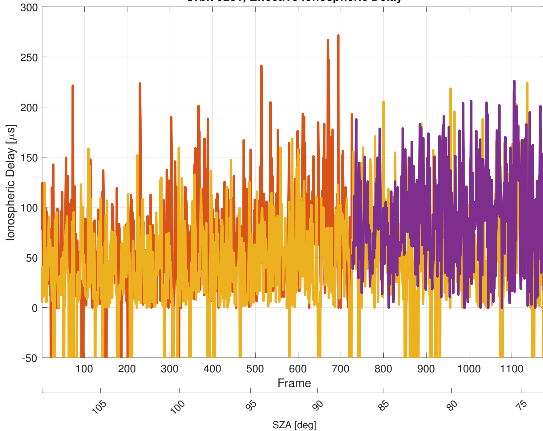
Orbit 9231, Effective Ionospheric Delay
