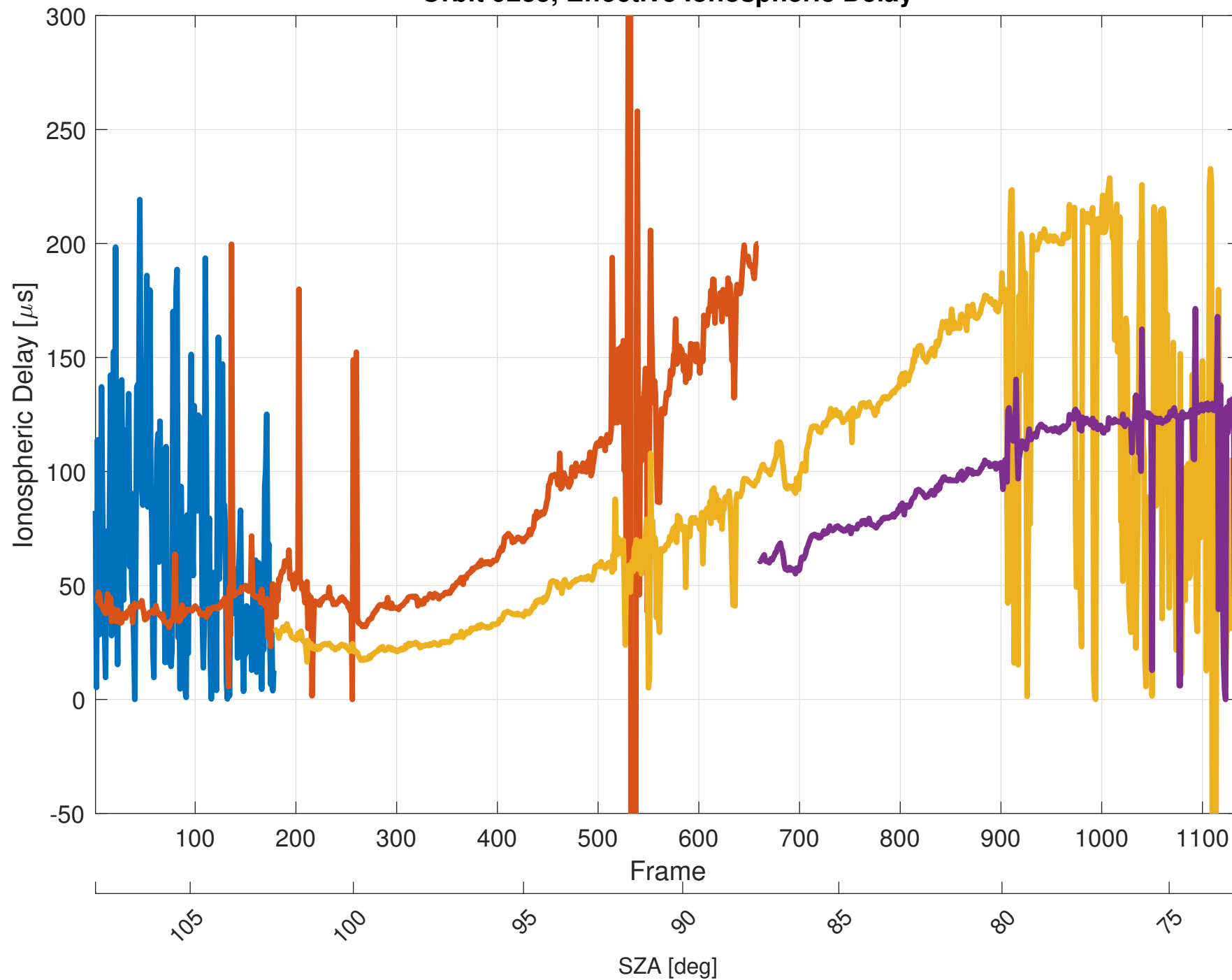
Orbit 9235, Effective Ionospheric Delay
