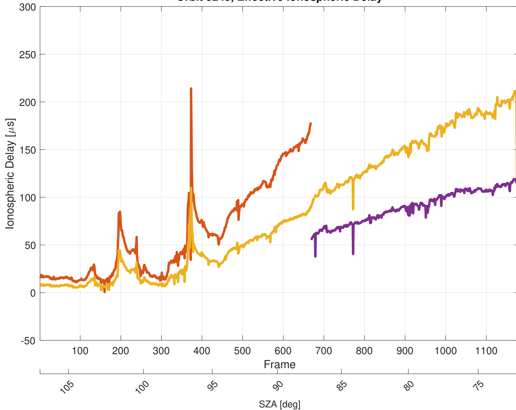
Orbit 9245, Effective Ionospheric Delay
