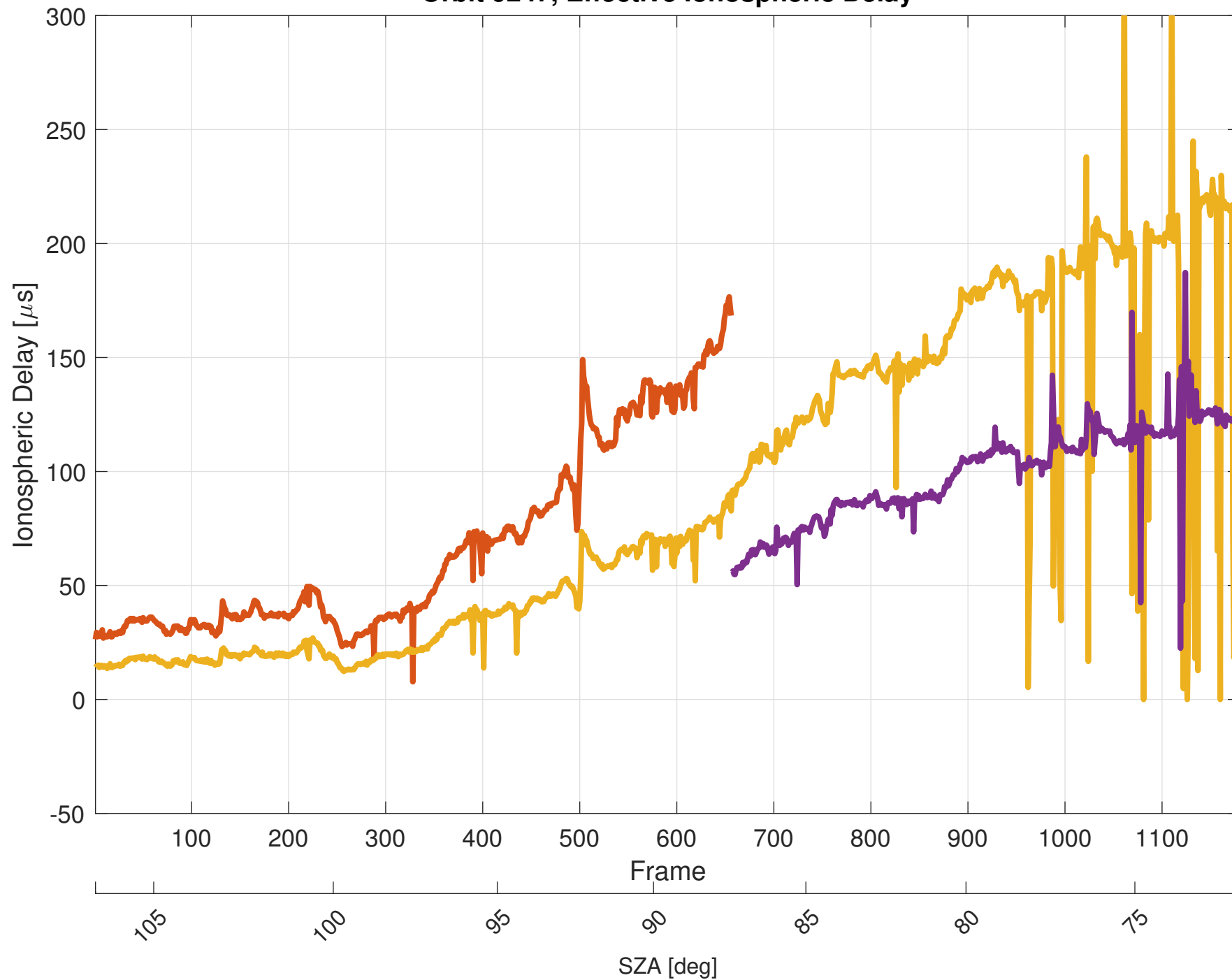
Orbit 9247, Effective Ionospheric Delay
