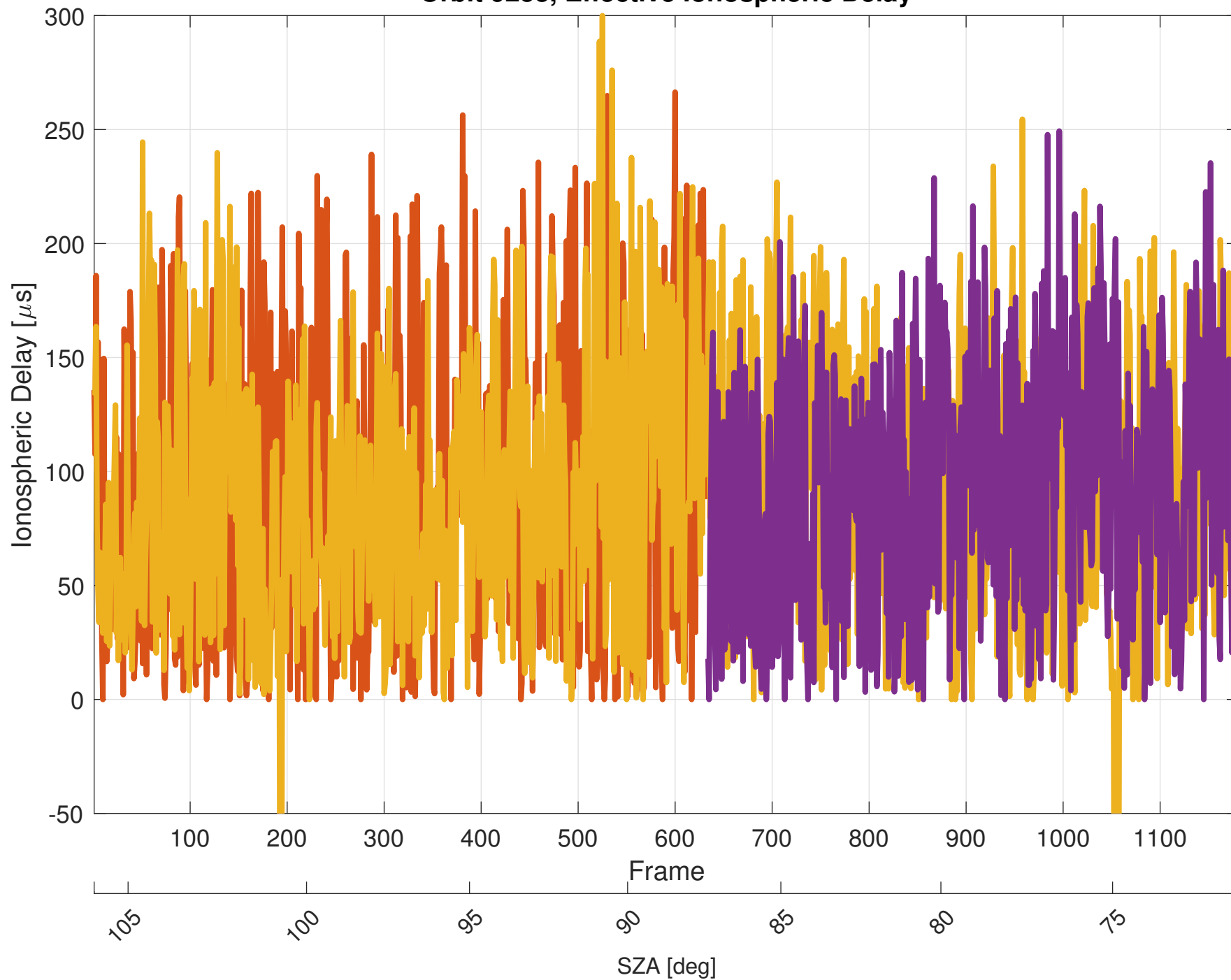
Orbit 9253, Effective Ionospheric Delay
