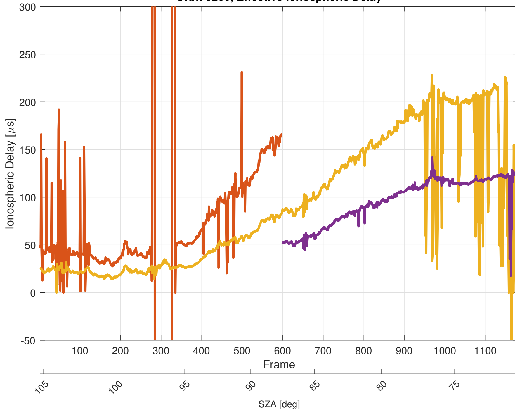
Orbit 9260, Effective Ionospheric Delay
