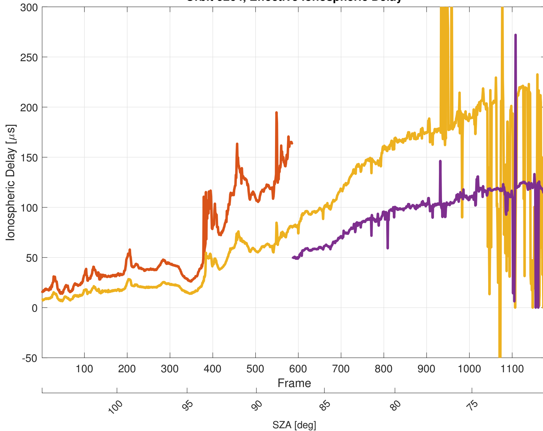
Orbit 9264, Effective Ionospheric Delay
