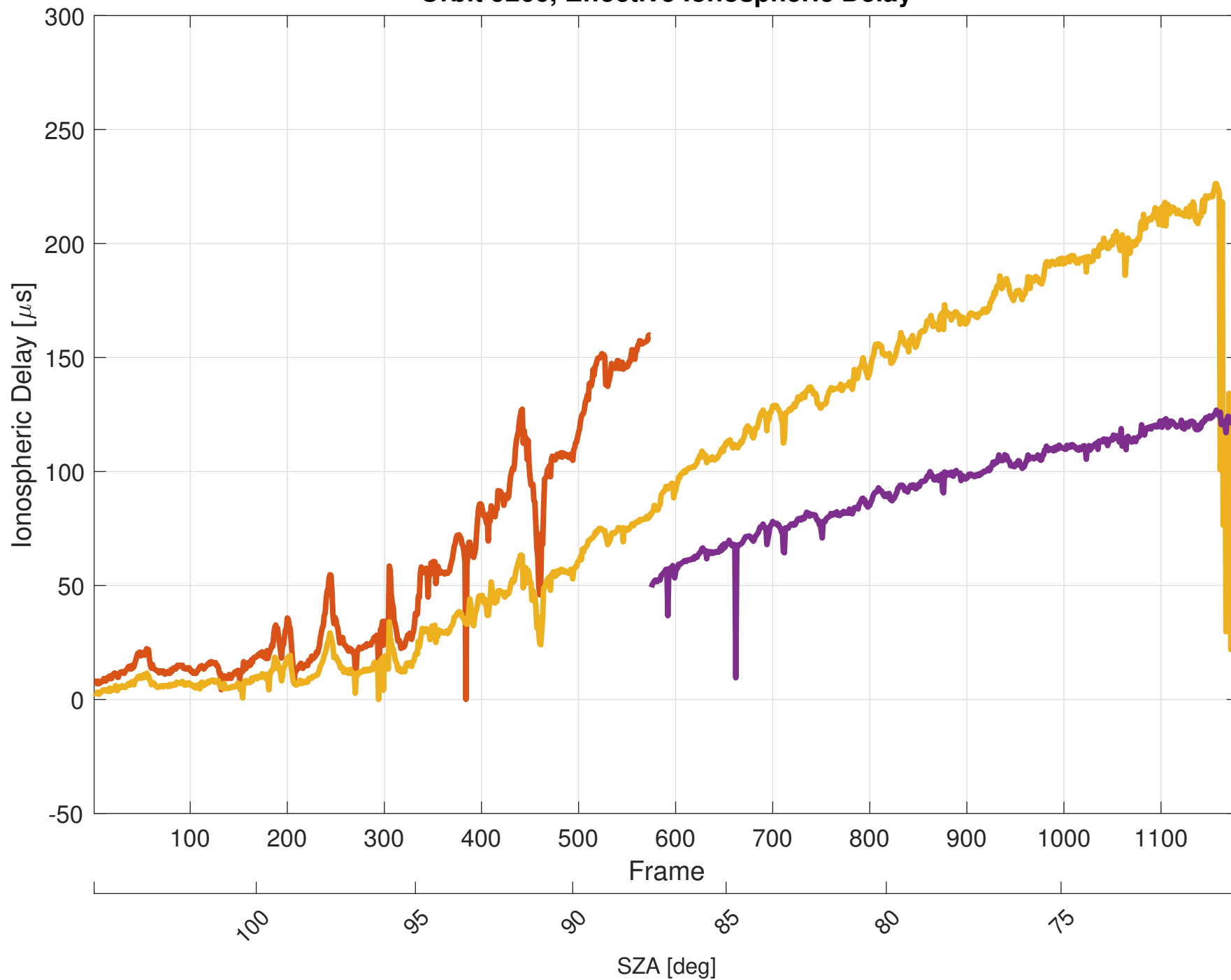
Orbit 9266, Effective Ionospheric Delay
