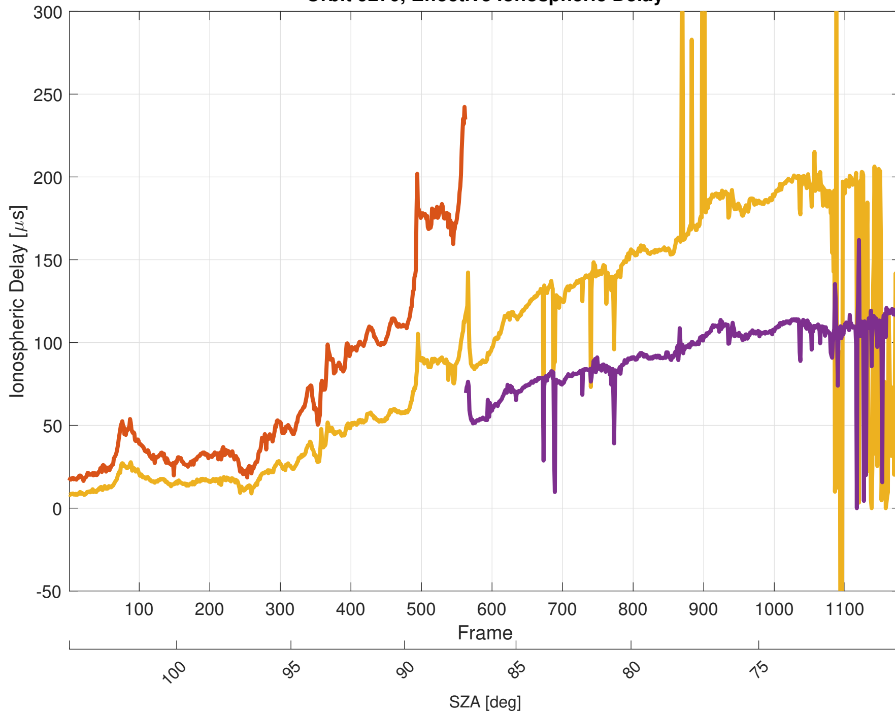
Orbit 9270, Effective Ionospheric Delay
