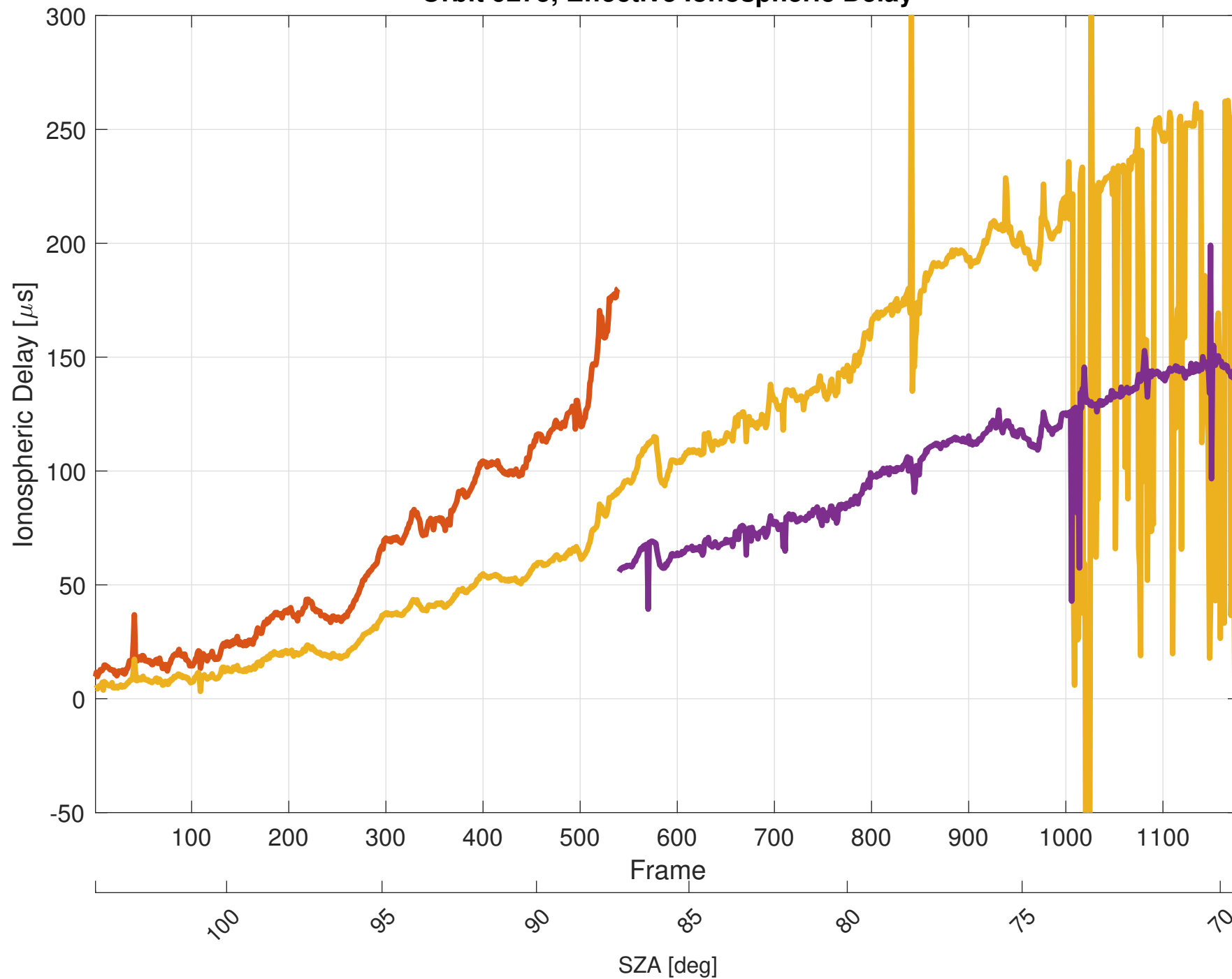
Orbit 9275, Effective Ionospheric Delay
