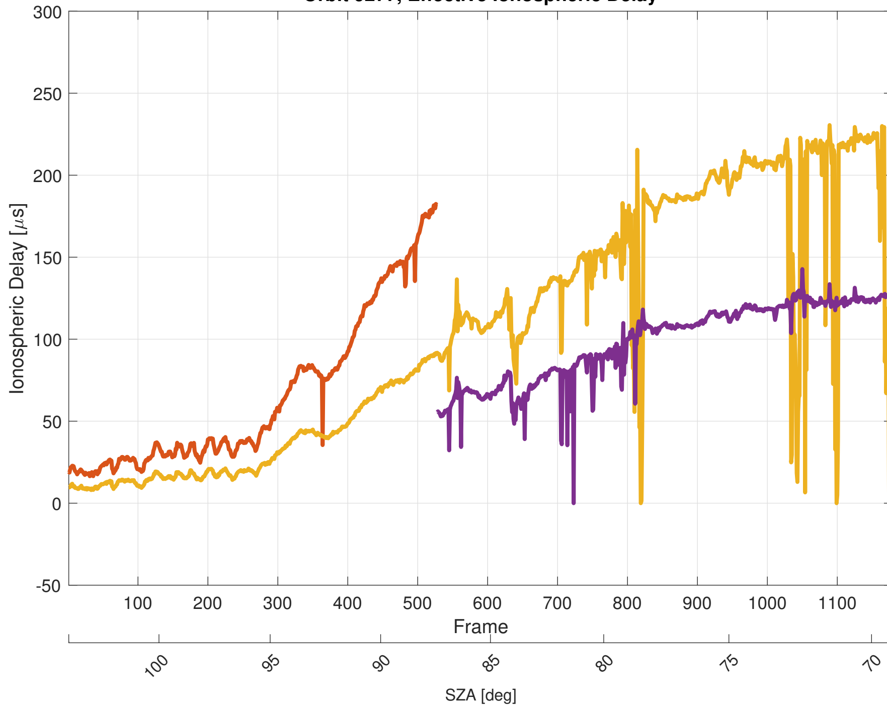
Orbit 9277, Effective Ionospheric Delay
