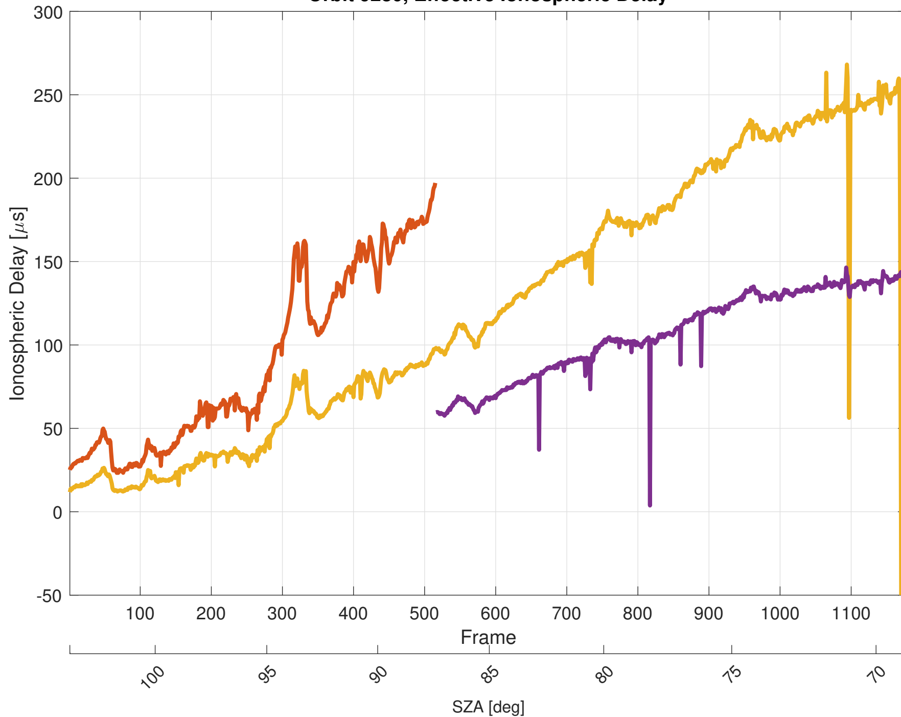
Orbit 9280, Effective Ionospheric Delay
