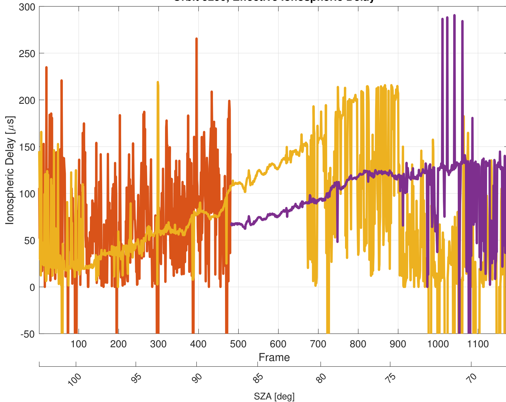
Orbit 9290, Effective Ionospheric Delay
