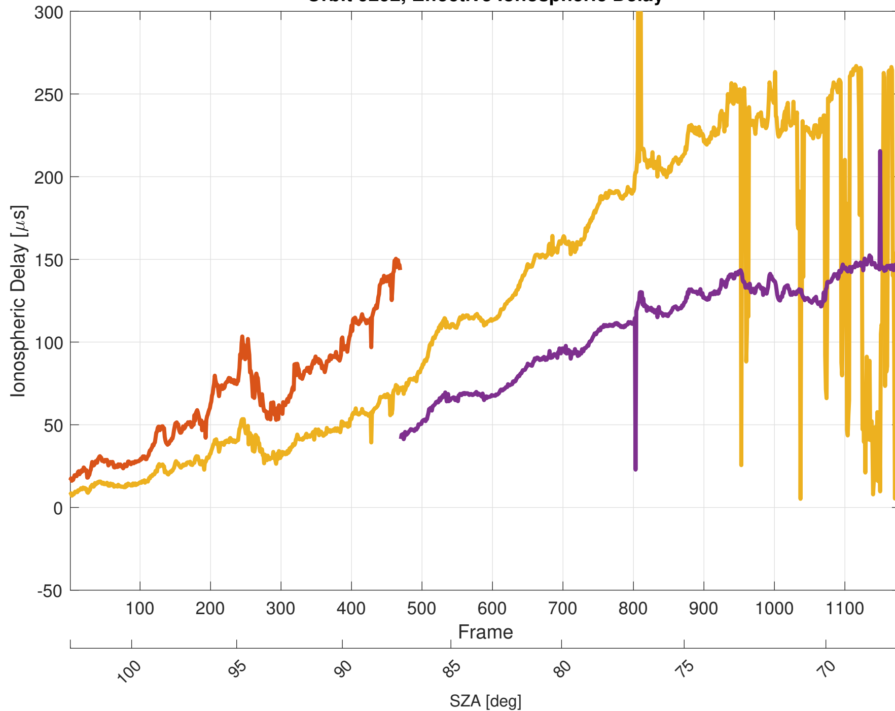
Orbit 9292, Effective Ionospheric Delay
