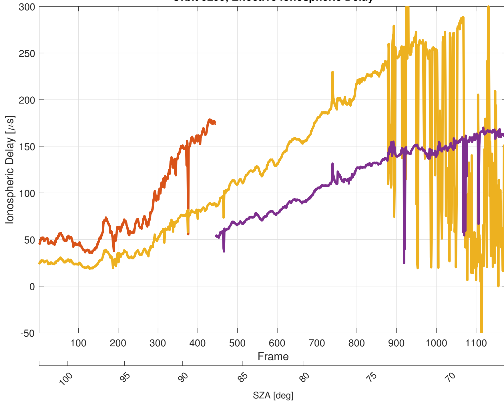
Orbit 9299, Effective Ionospheric Delay
