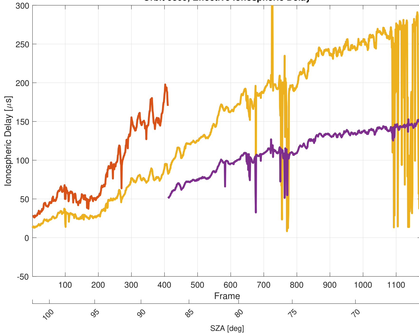
Orbit 9309, Effective Ionospheric Delay
