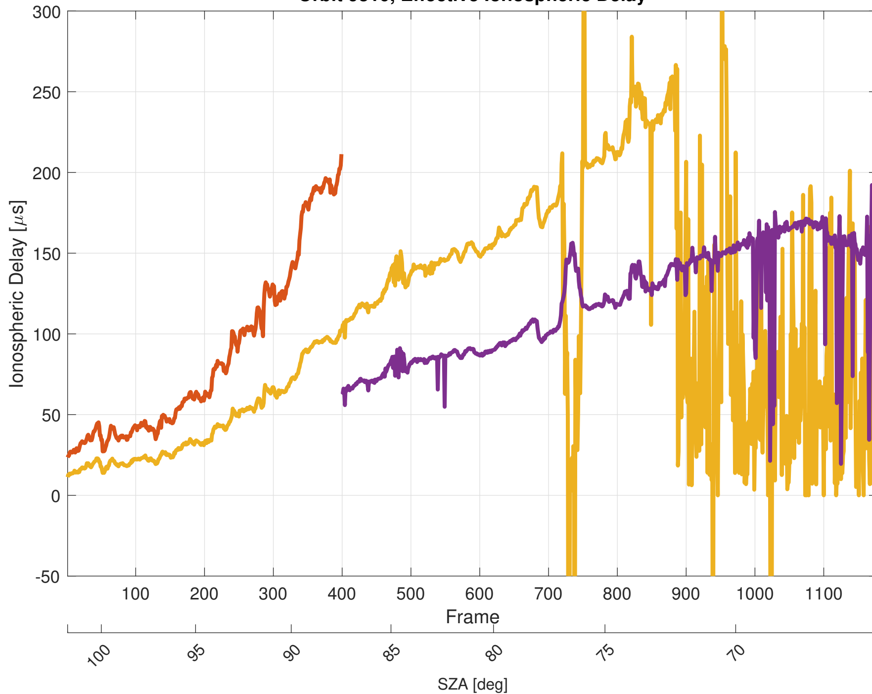
Orbit 9310, Effective Ionospheric Delay
