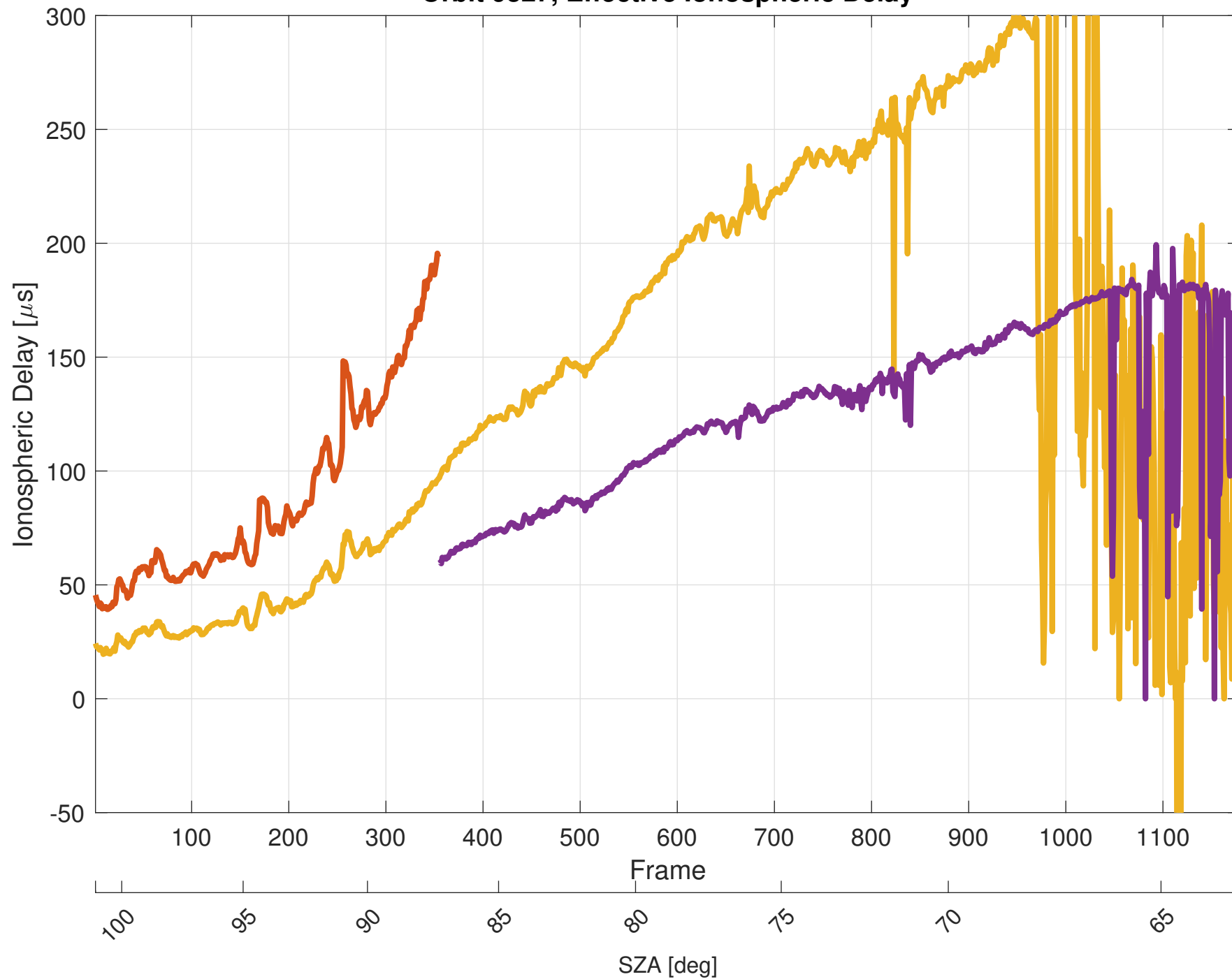
Orbit 9327, Effective Ionospheric Delay
