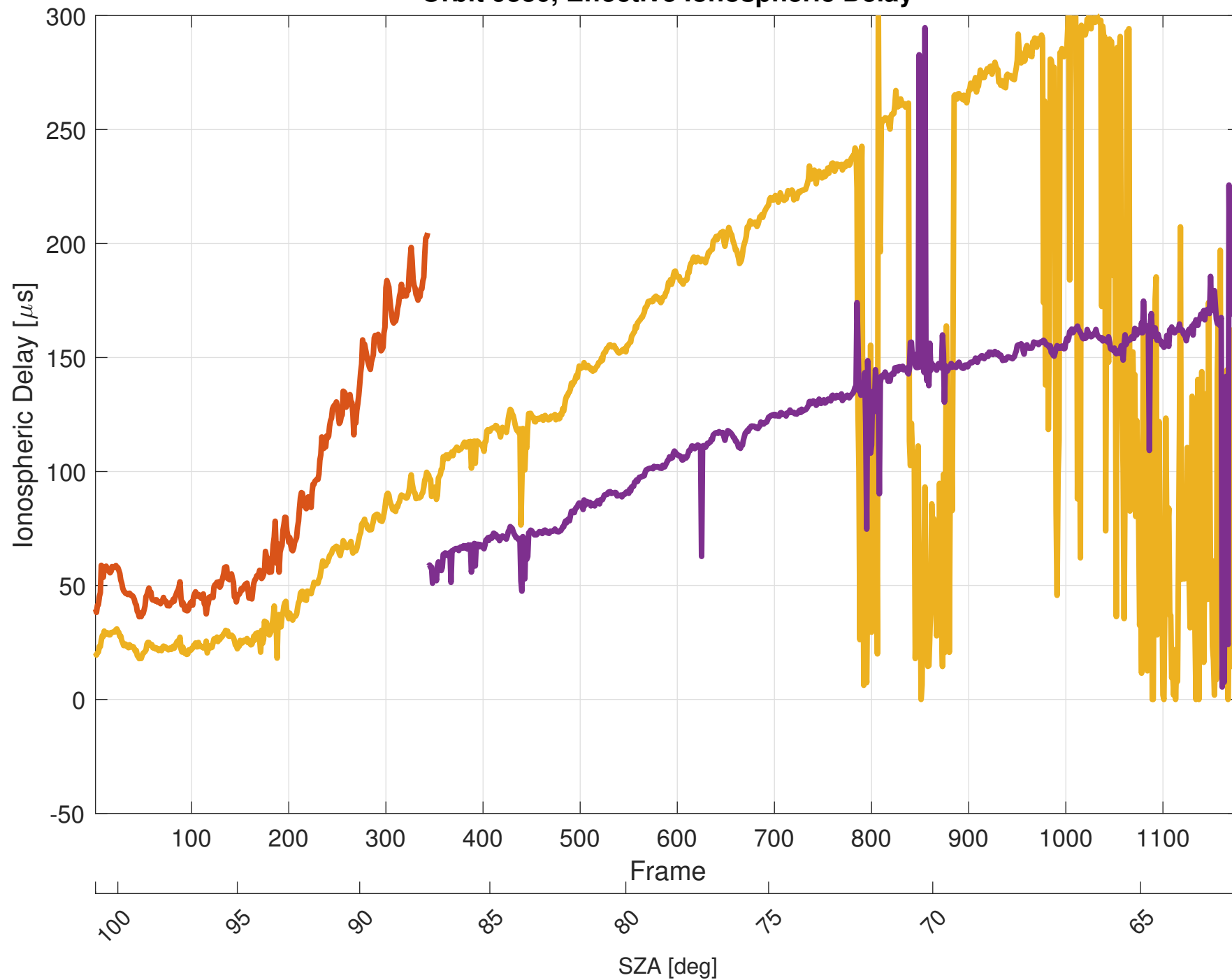
Orbit 9330, Effective Ionospheric Delay
