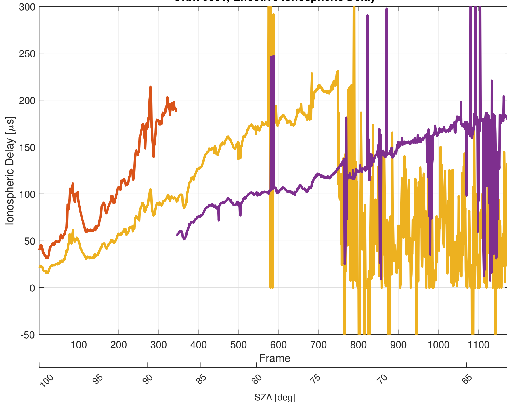
Orbit 9331, Effective Ionospheric Delay
