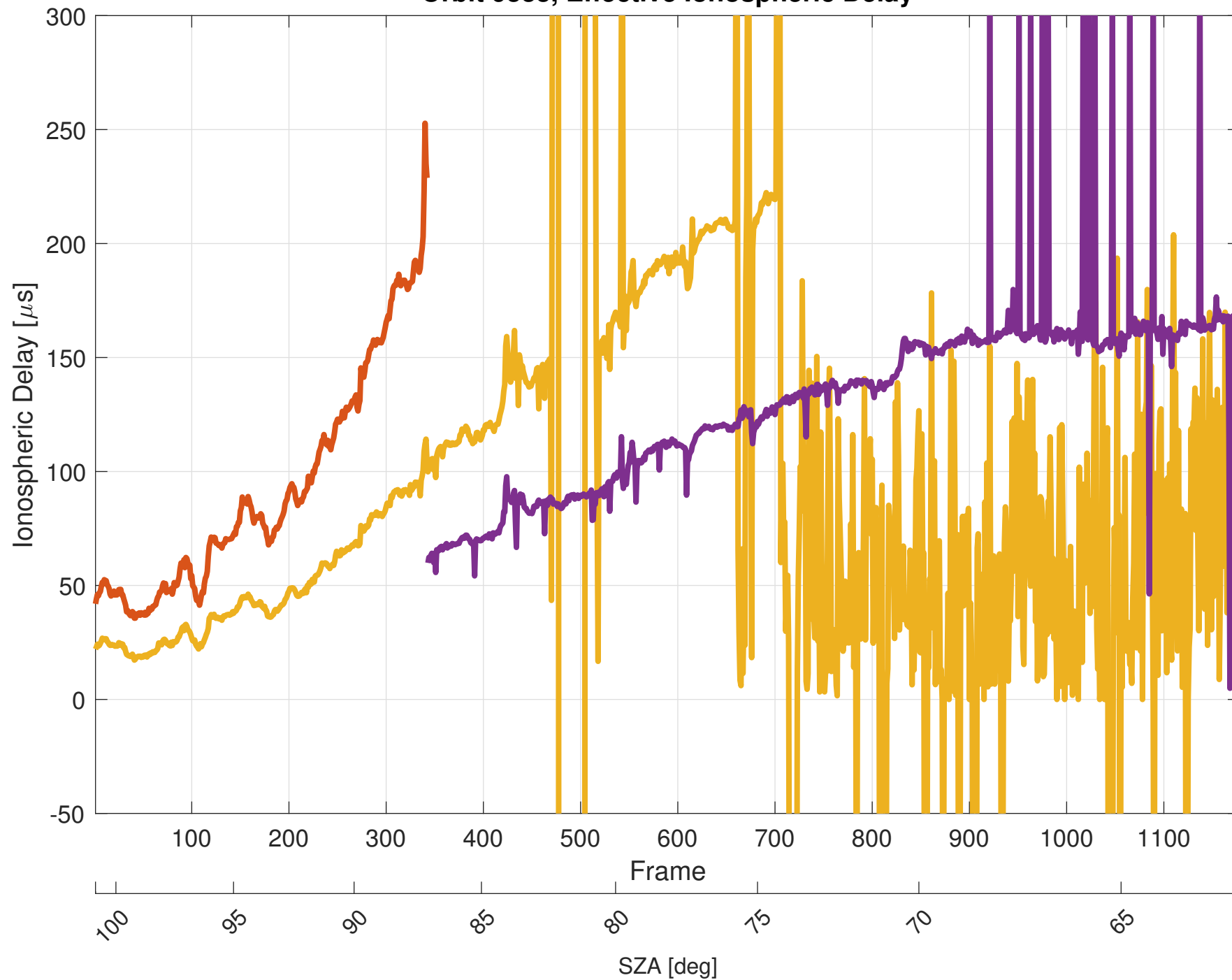
Orbit 9333, Effective Ionospheric Delay
