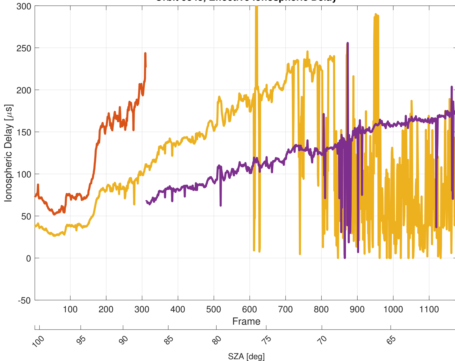
Orbit 9343, Effective Ionospheric Delay
